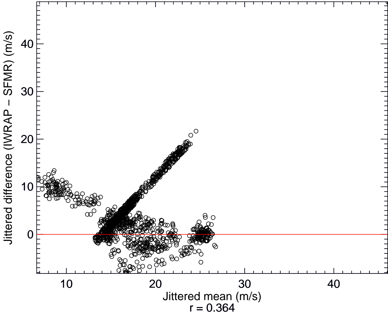
Mean-Difference Plot of IWRAP HH vs. SFMR Wind Speed
