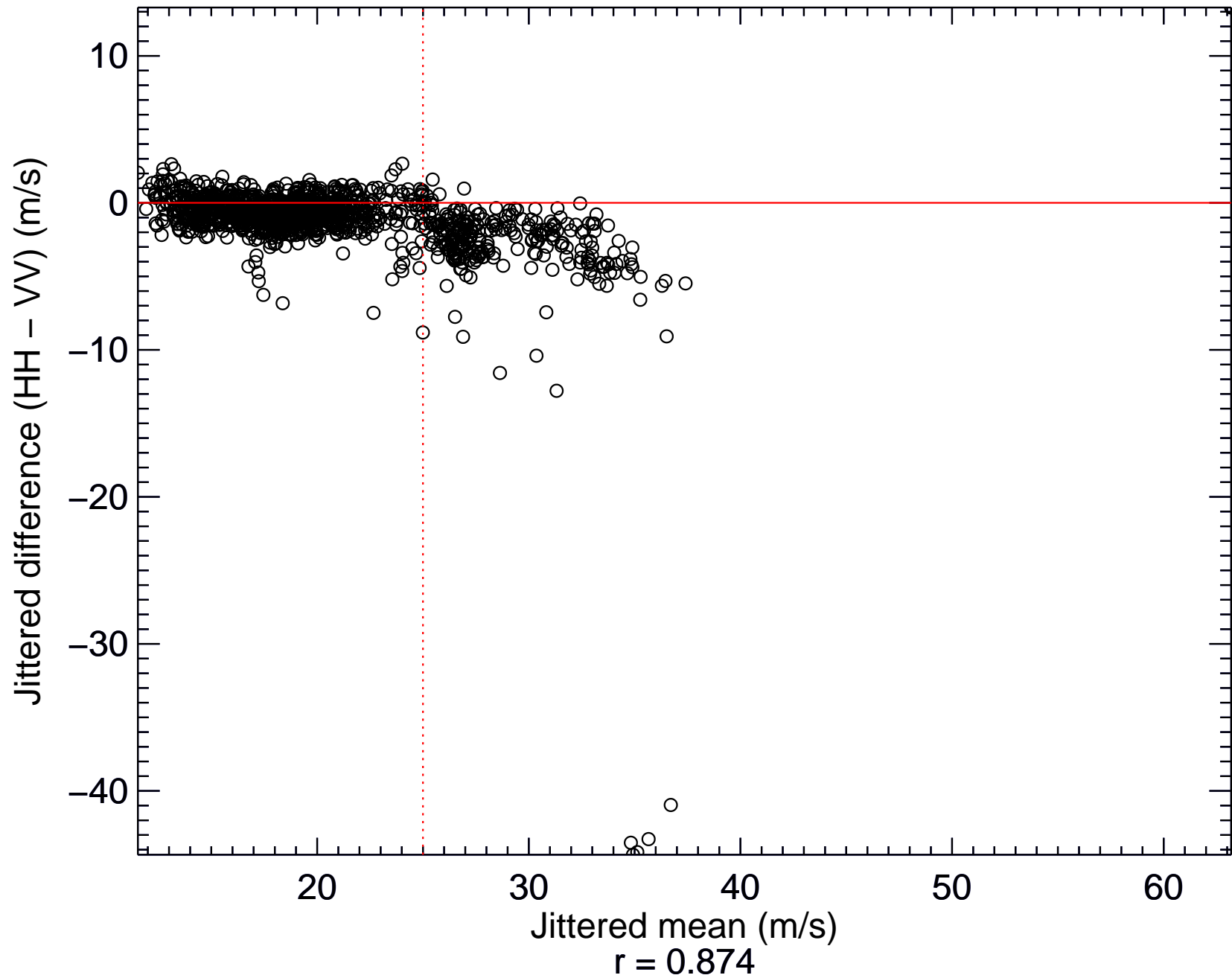
Mean-Difference Plot of IWRAP VV vs. IWRAP HH Wind Speed
