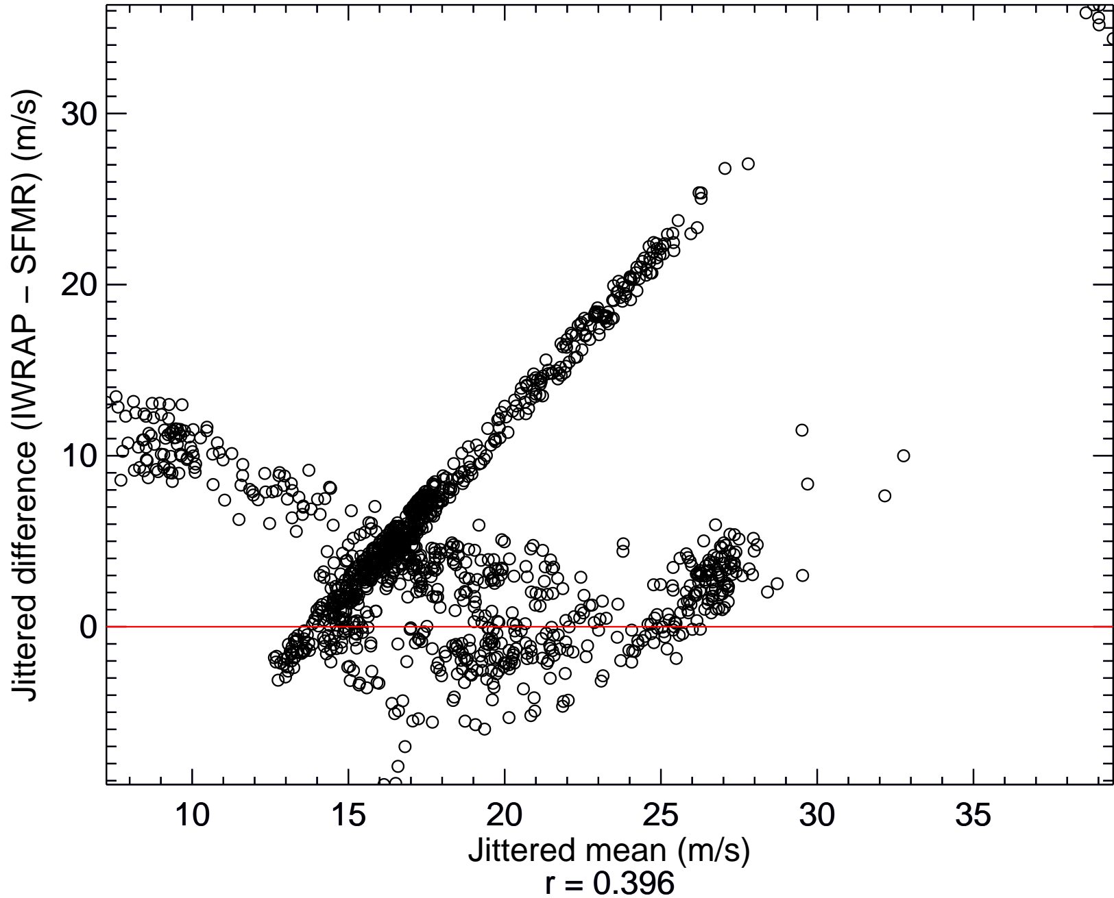
Mean-Difference Plot of IWRAP VV vs. SFMR Wind Speed
