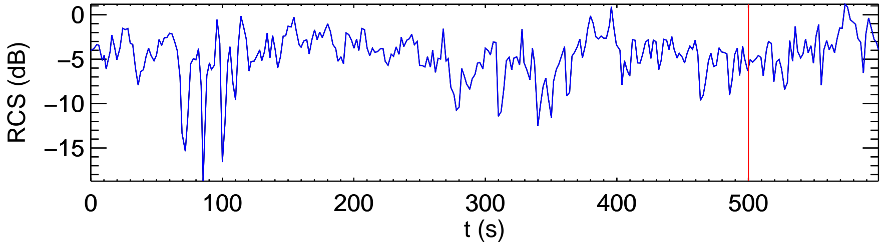
C-band RCS
