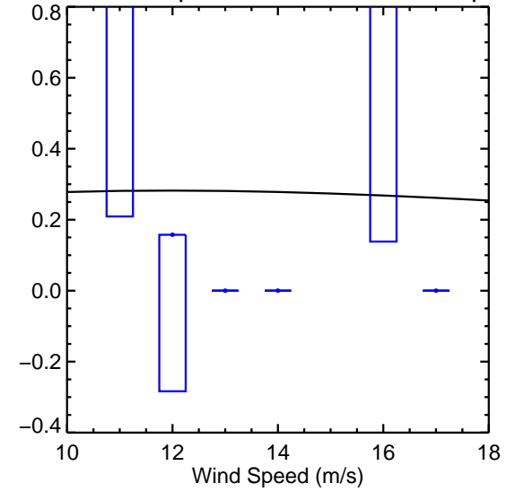
C-band VV-pol a2 vs. SFMR Wind Speed
