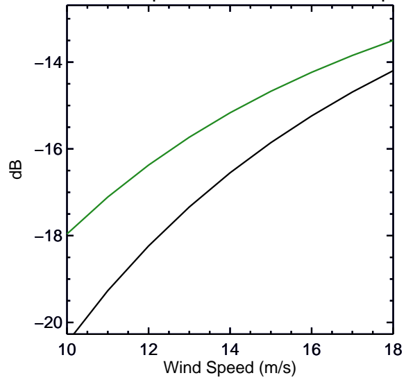
C-band VV-pol A0 vs. SFMR Wind Speed
