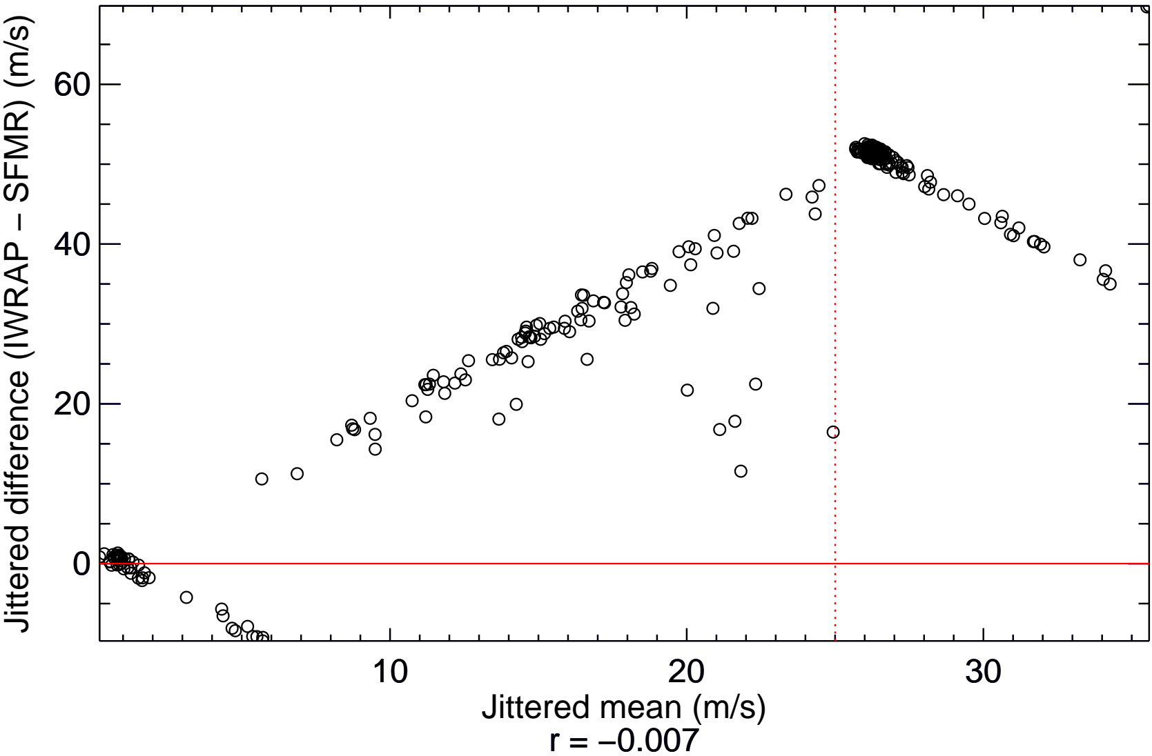
Mean-Difference Plot of IWRAP VV and SFMR Wind Speed
