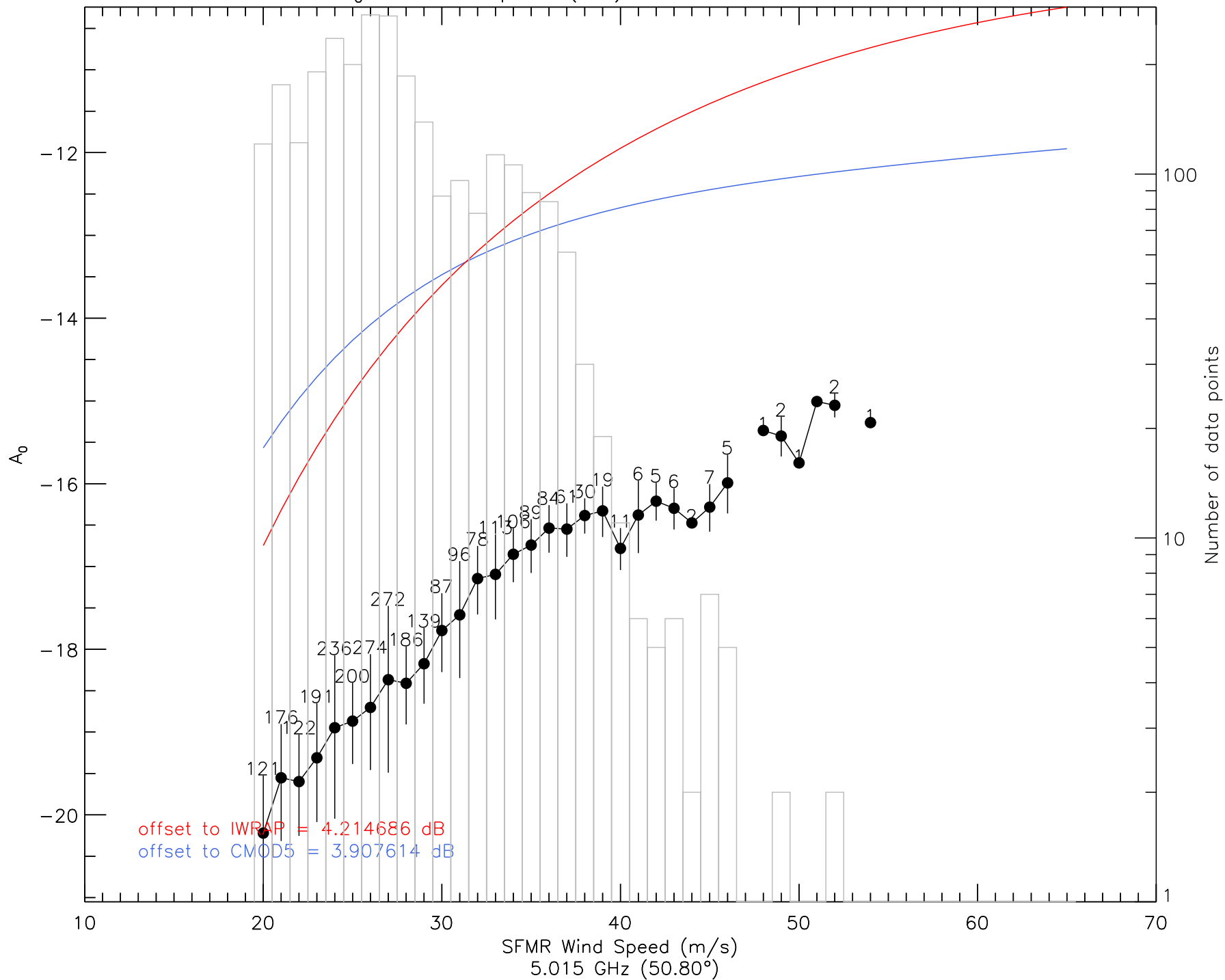
A_0 vs. Wind Speed (I2a) – uc1 20090819 hws
