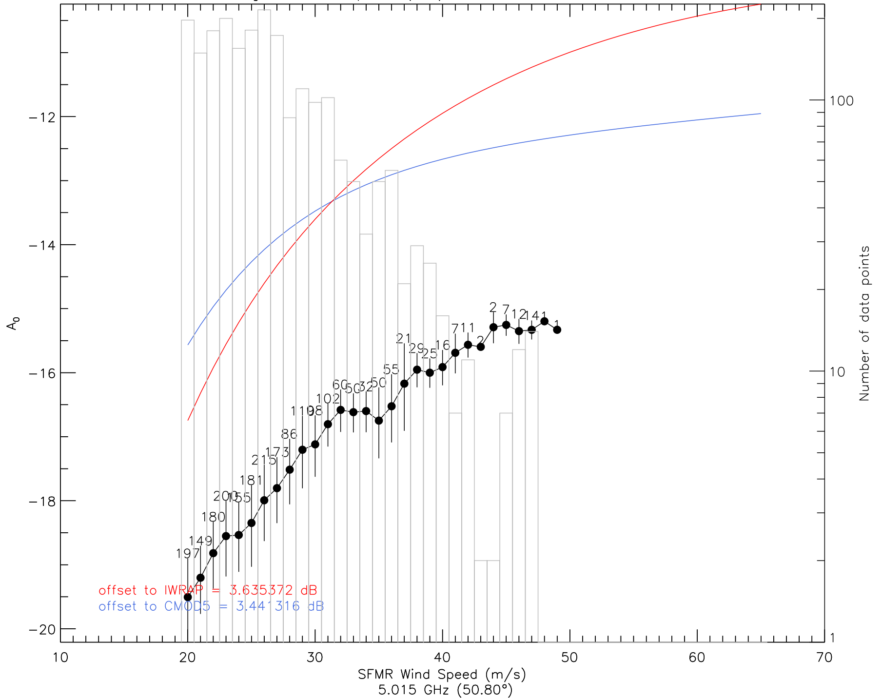
A_0 vs. Wind Speed (I2a) – uc1 20090820 hws
