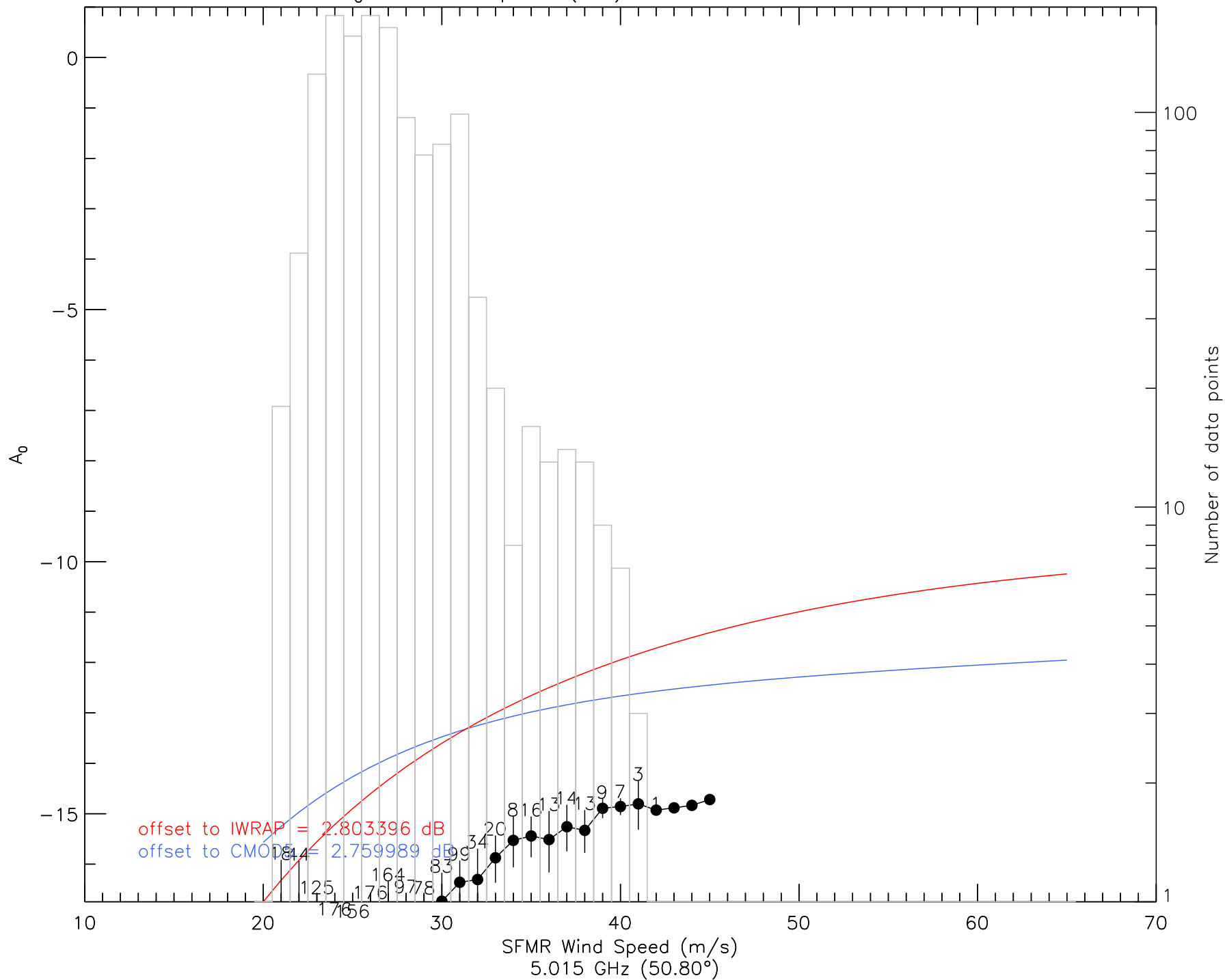
A_0 vs. Wind Speed (I2a) – uc1 20090821 hws
