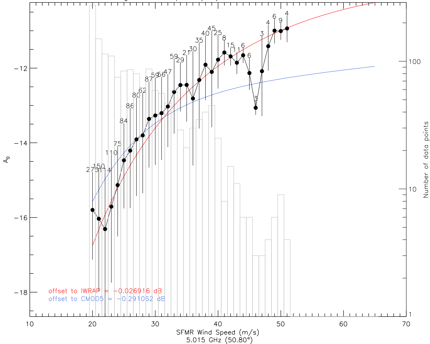
A_0 vs. Wind Speed (12a) – uc1 20090818 hws
