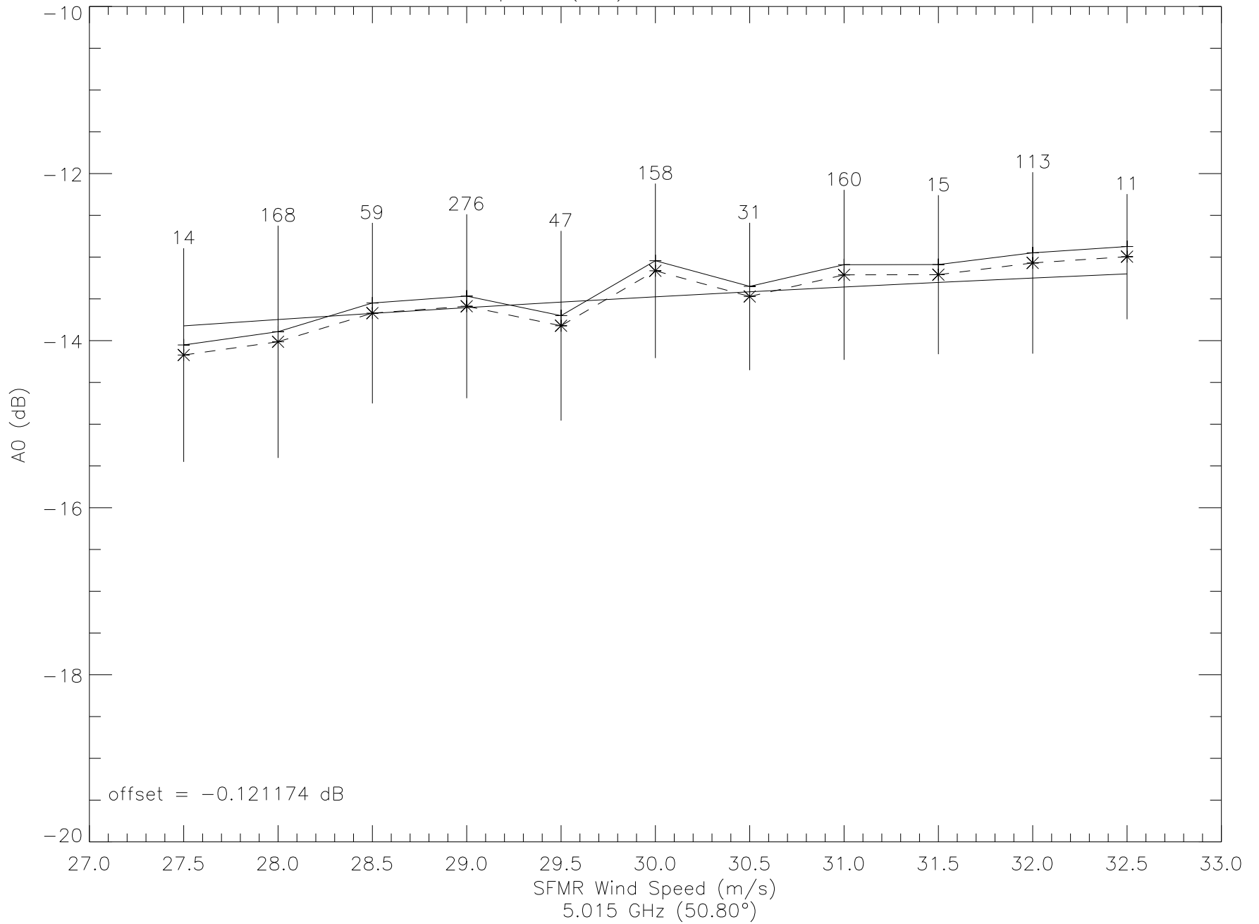
A0 vs. Wind Speed (I1b) - IW20090818212108Z.uc1
