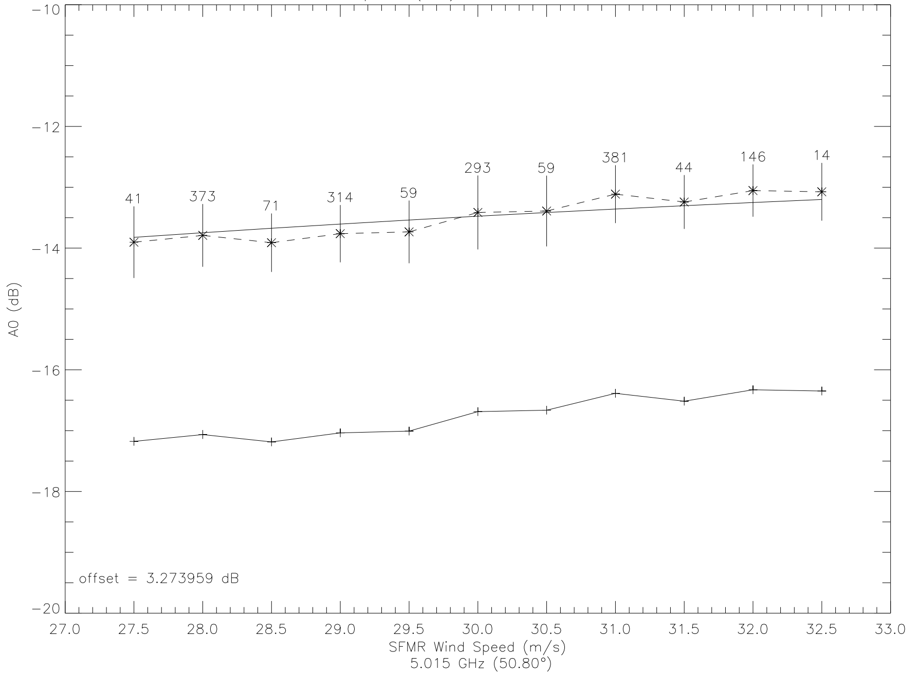
A0 vs. Wind Speed (I1b) - IW20090820233416Z.uc1
