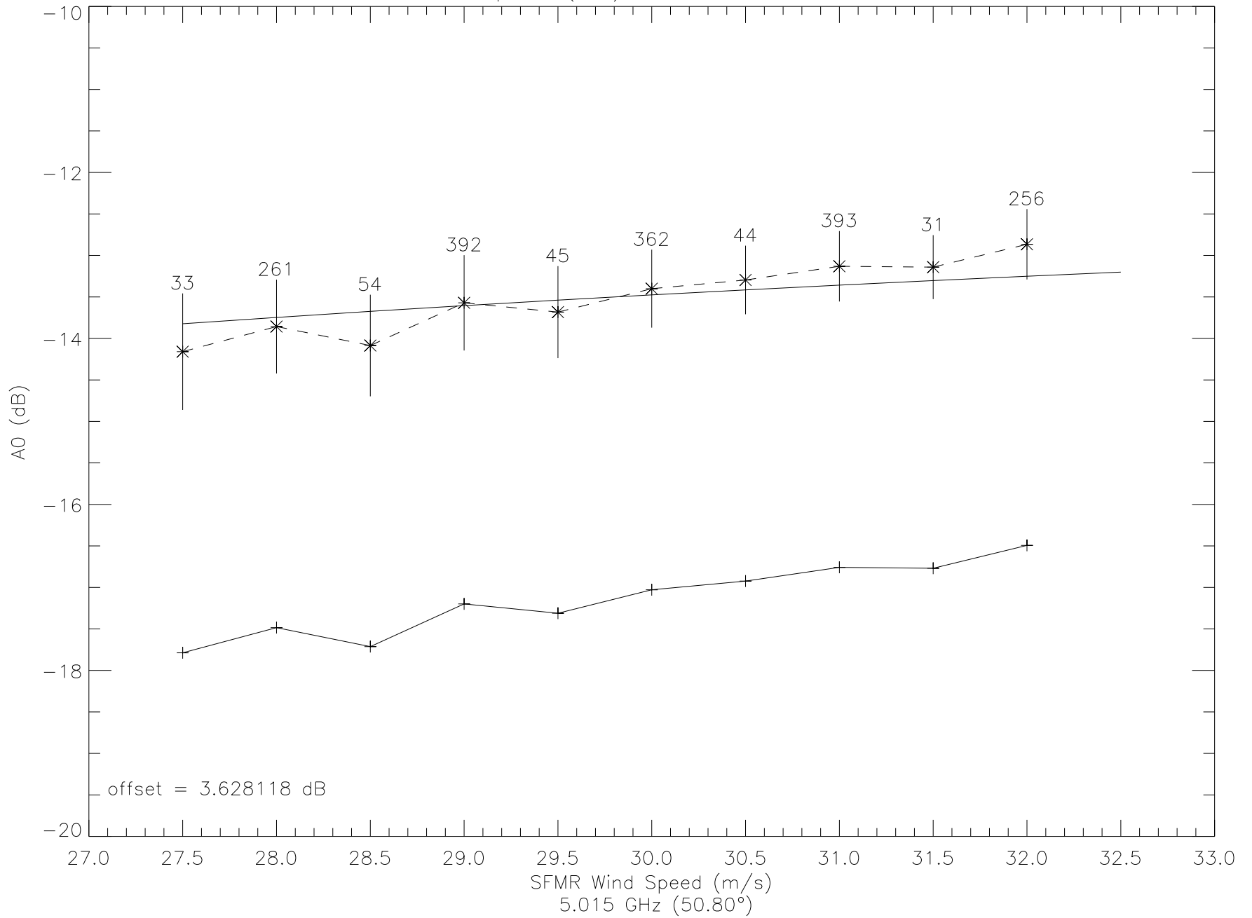
A0 vs. Wind Speed (I1b) - IW20090820090837Z.uc1
