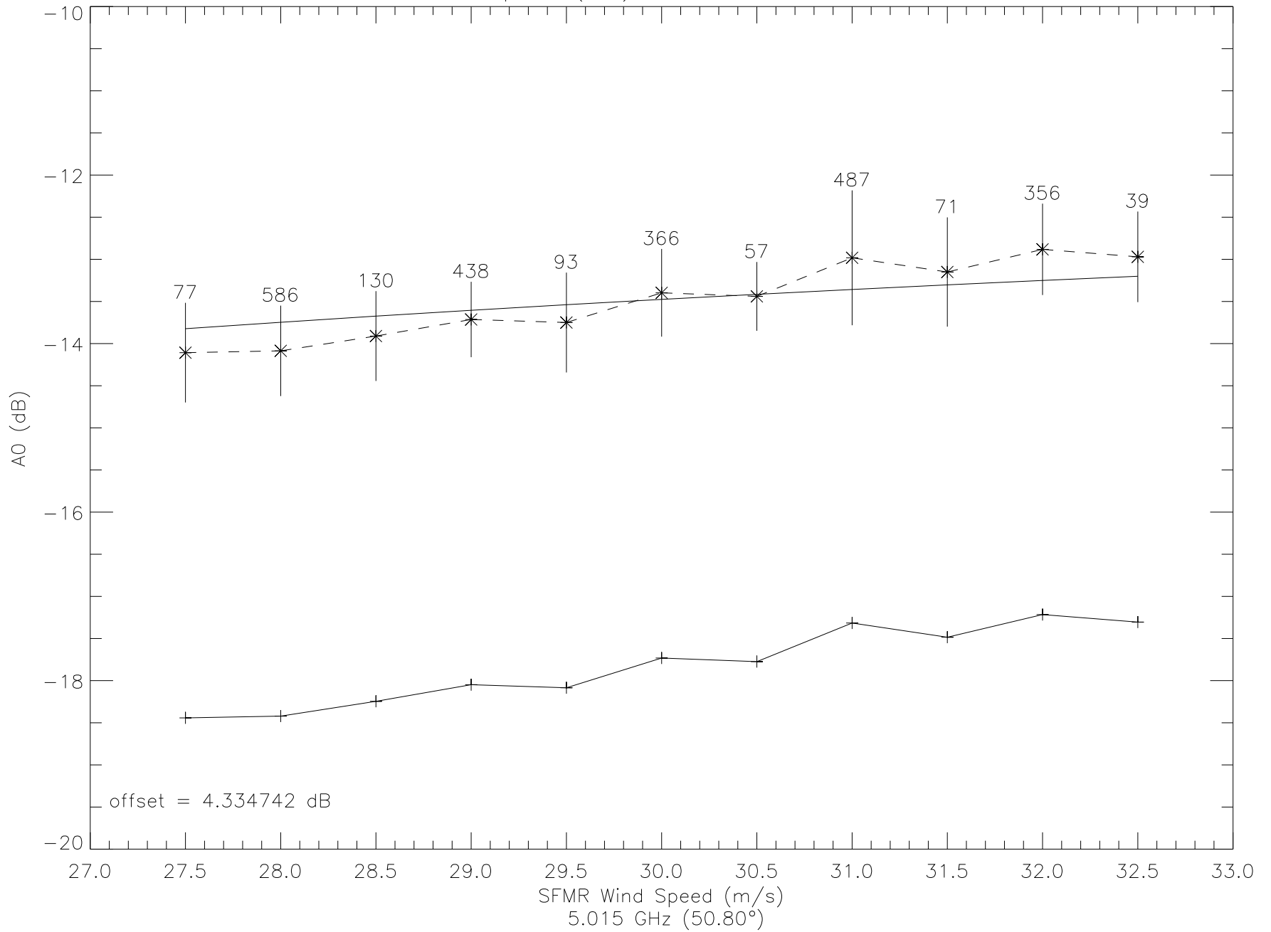
A0 vs. Wind Speed (I1b) - IW20090819083110Z.uc1
