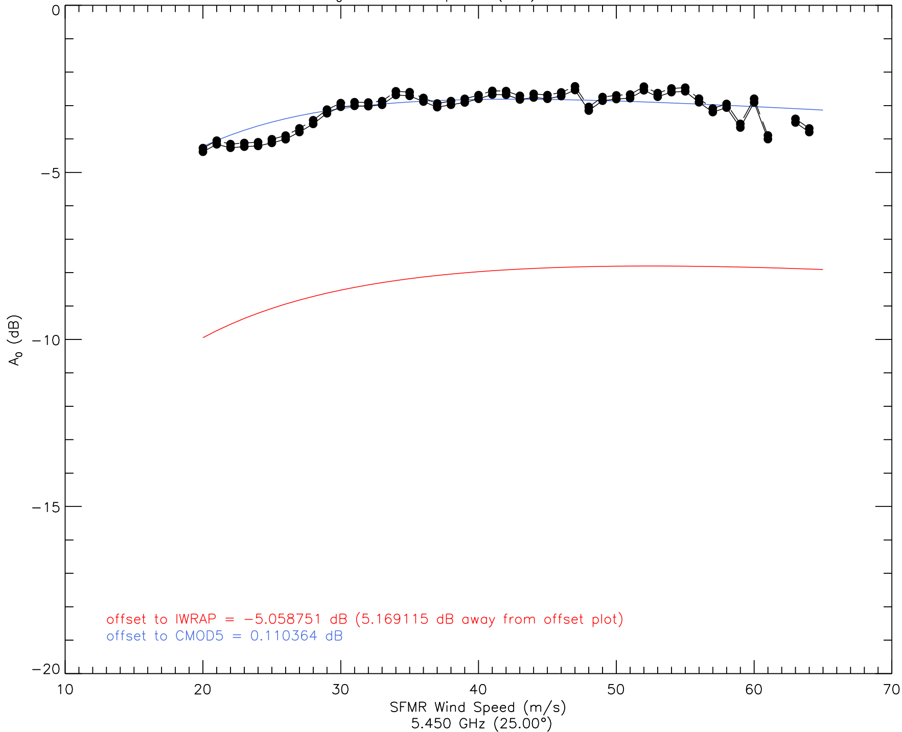
A_0 vs. Wind Speed (I1b) - All uc2
