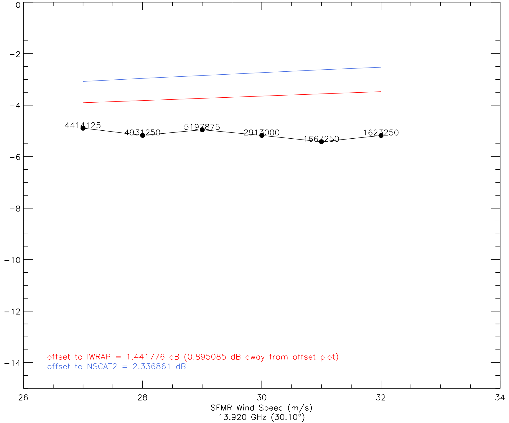
A_0 vs. Wind Speed (I2a) - 20080911 - ku2
