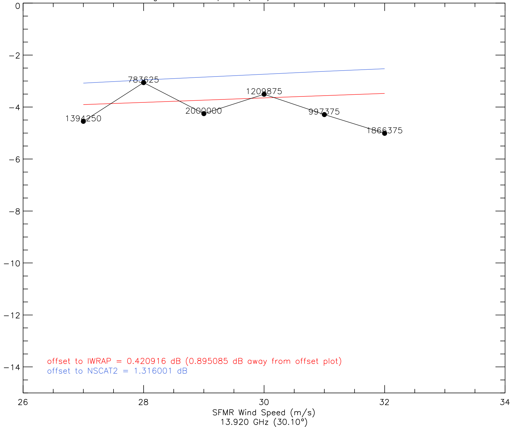
A_0 vs. Wind Speed (I2a) - 20080912 - ku2
