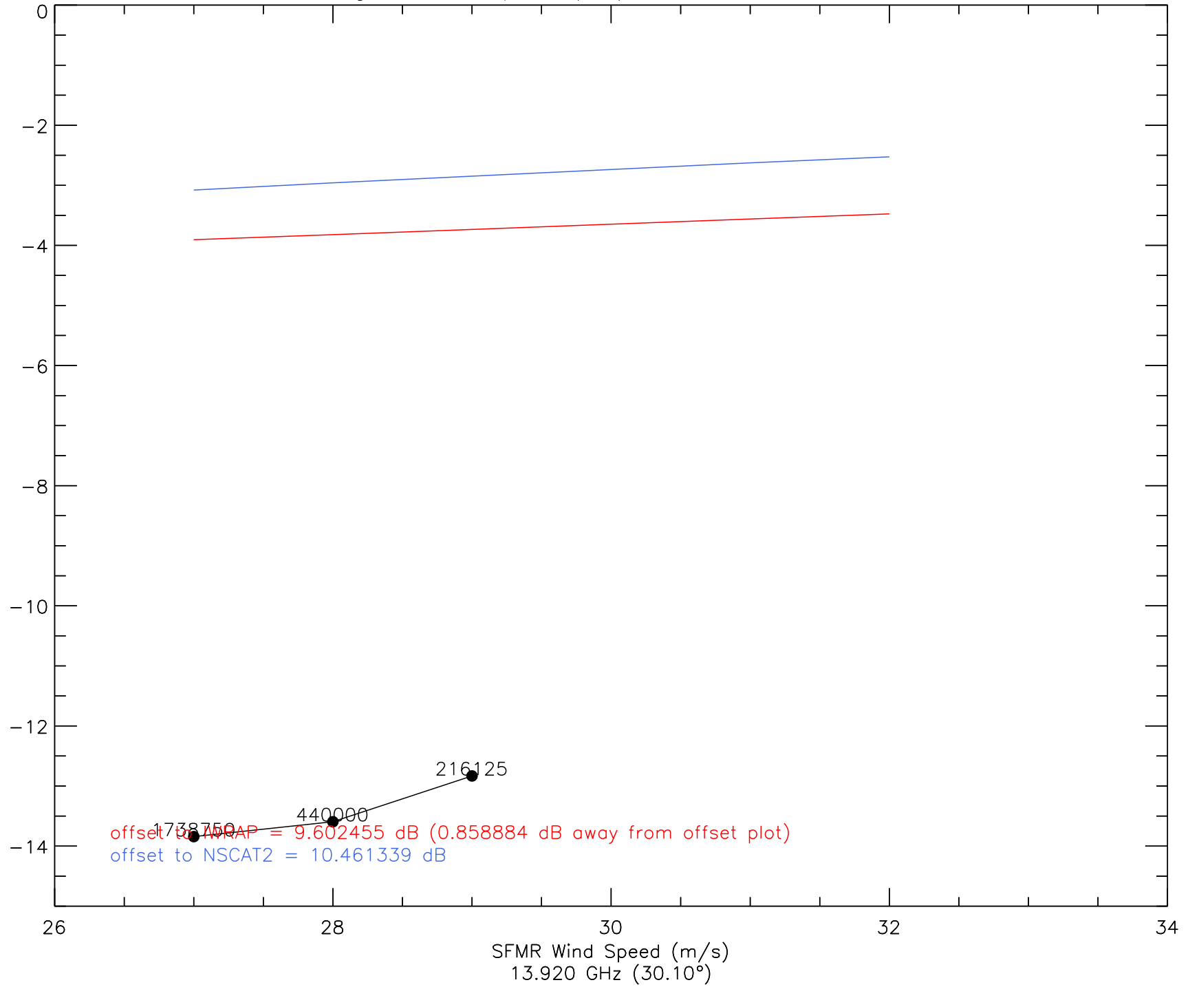
A_0 vs. Wind Speed (I2a) - 20080925 - ku2
