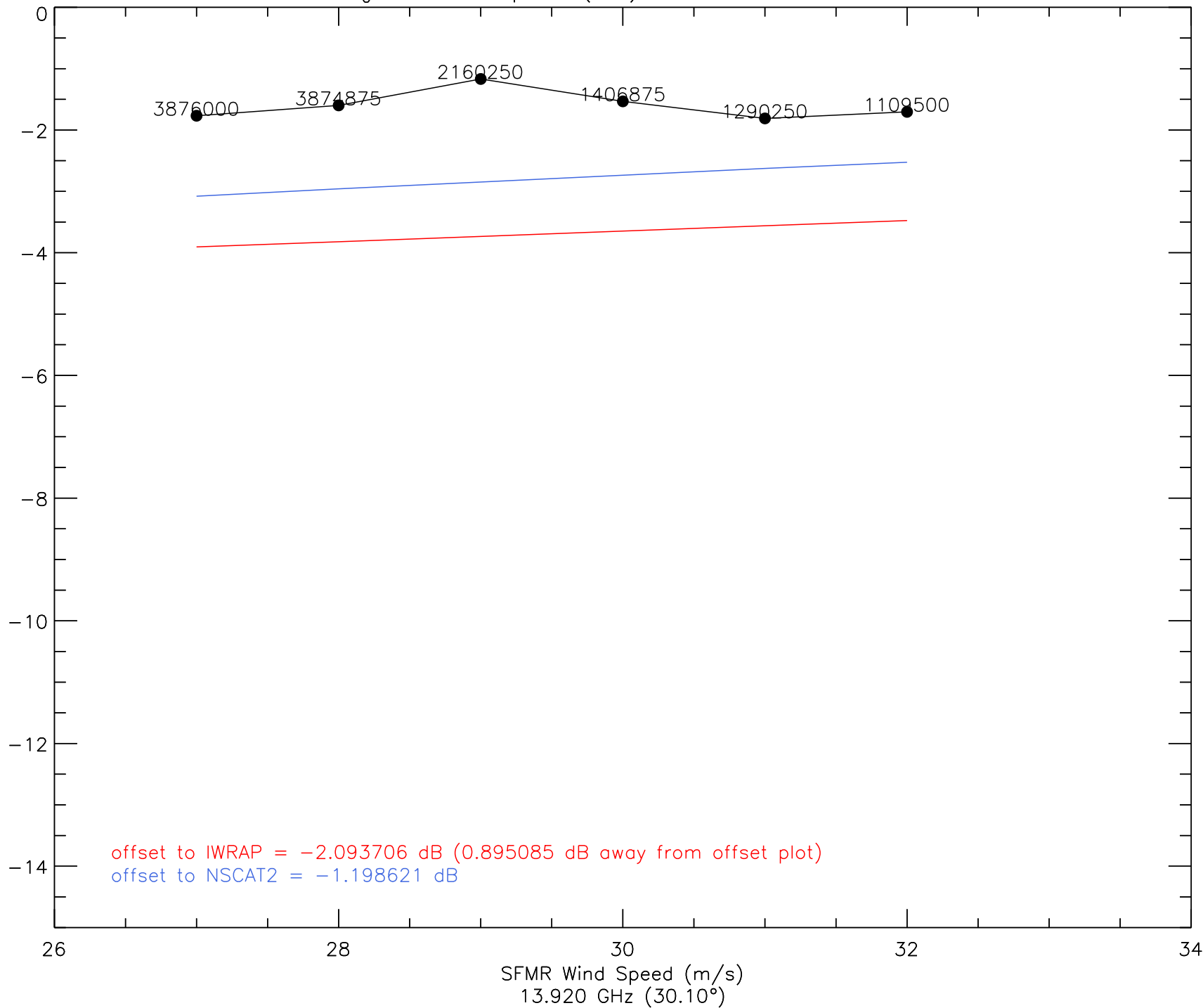
A_0 vs. Wind Speed (I2a) - 20080829 - ku2
