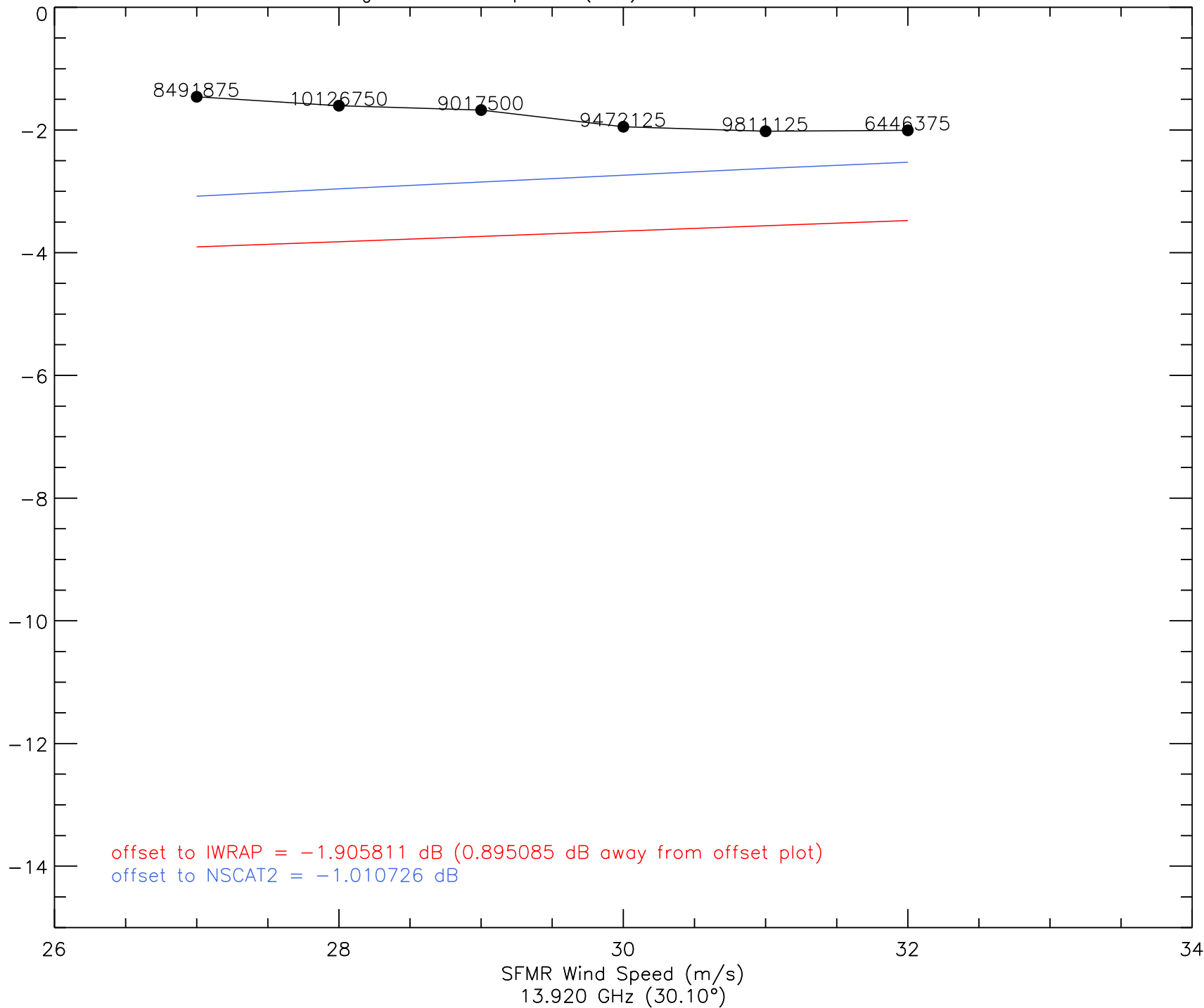
A_0 vs. Wind Speed (I2a) - 20080906 - ku2
