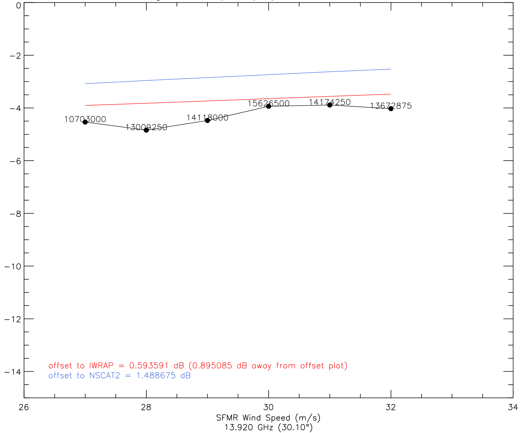
A_0 vs. Wind Speed (I2a) - 20080831 - ku2
