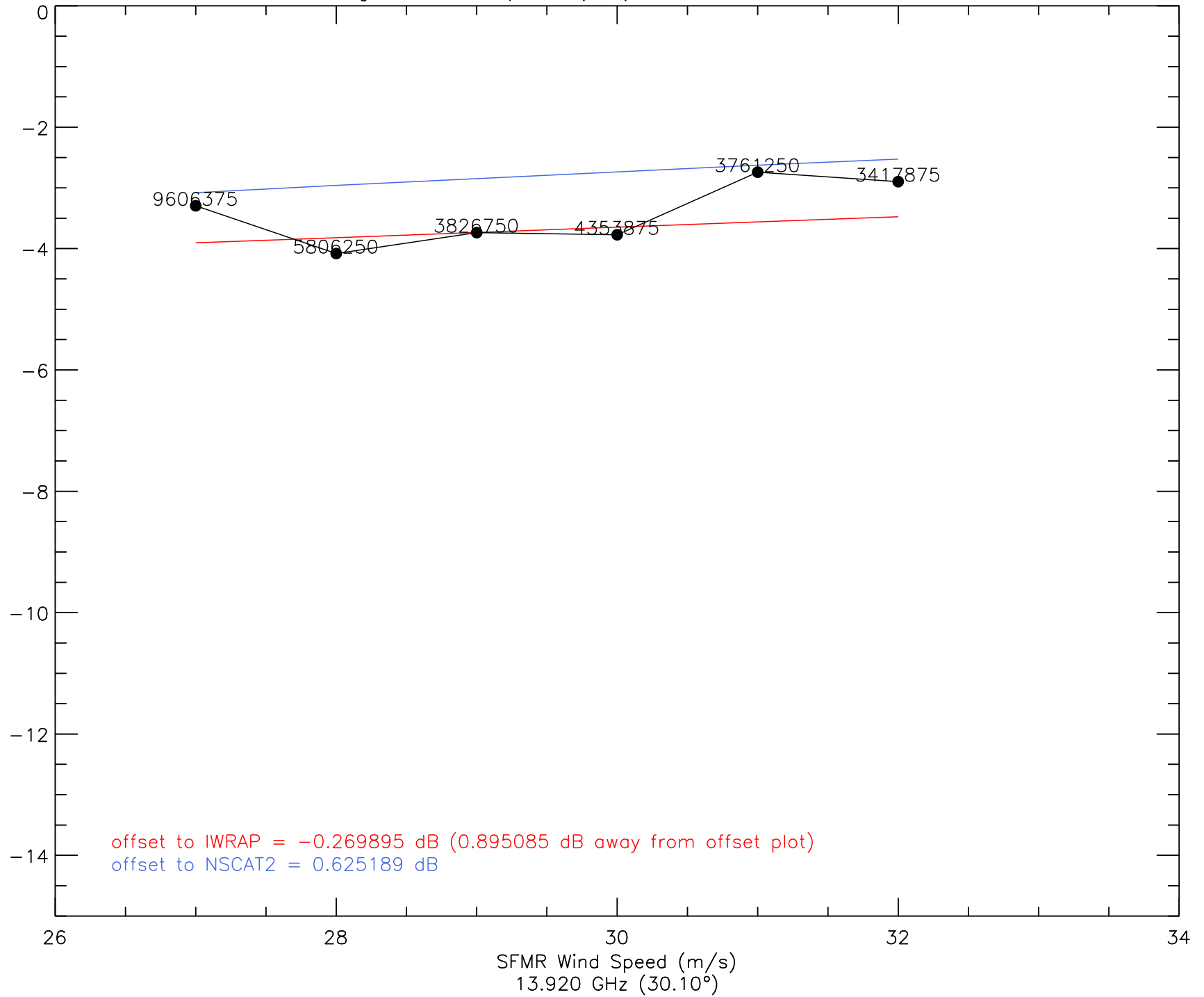
A_0 vs. Wind Speed (I2a) - 20080830 - ku2
