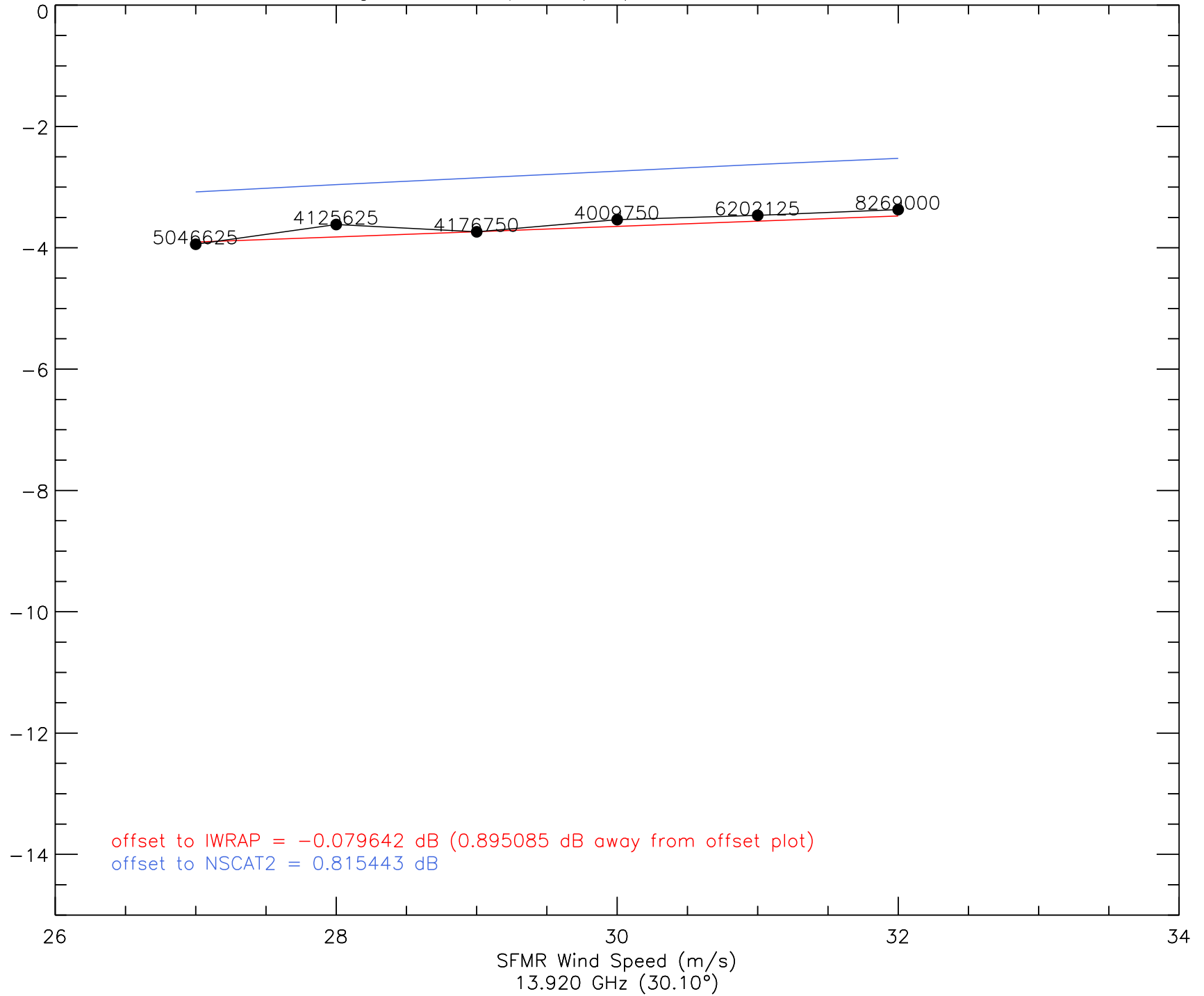
A_0 vs. Wind Speed (I2a) - 20080907 - ku2
