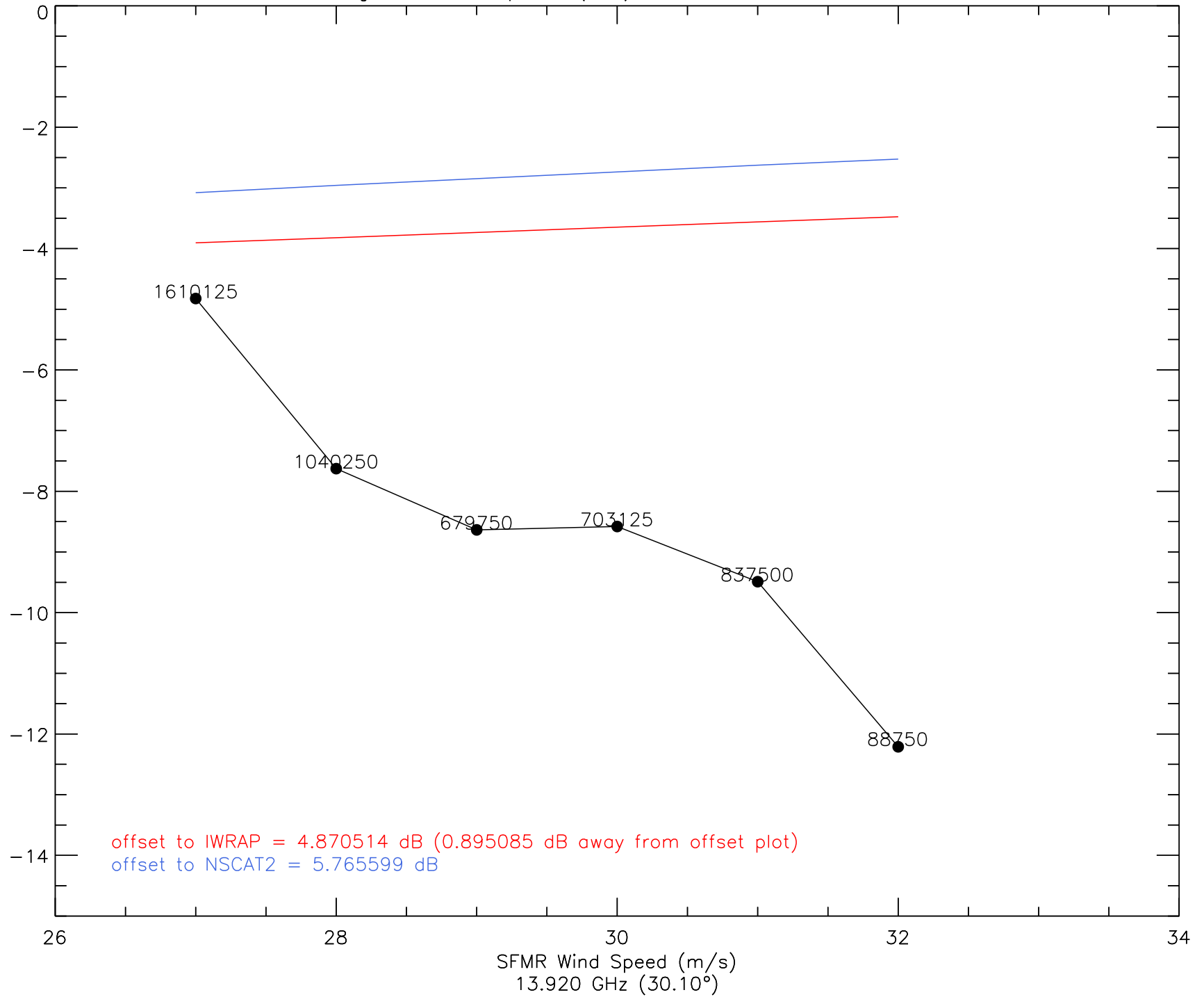
A_0 vs. Wind Speed (I2a) - 20080909 - ku2
