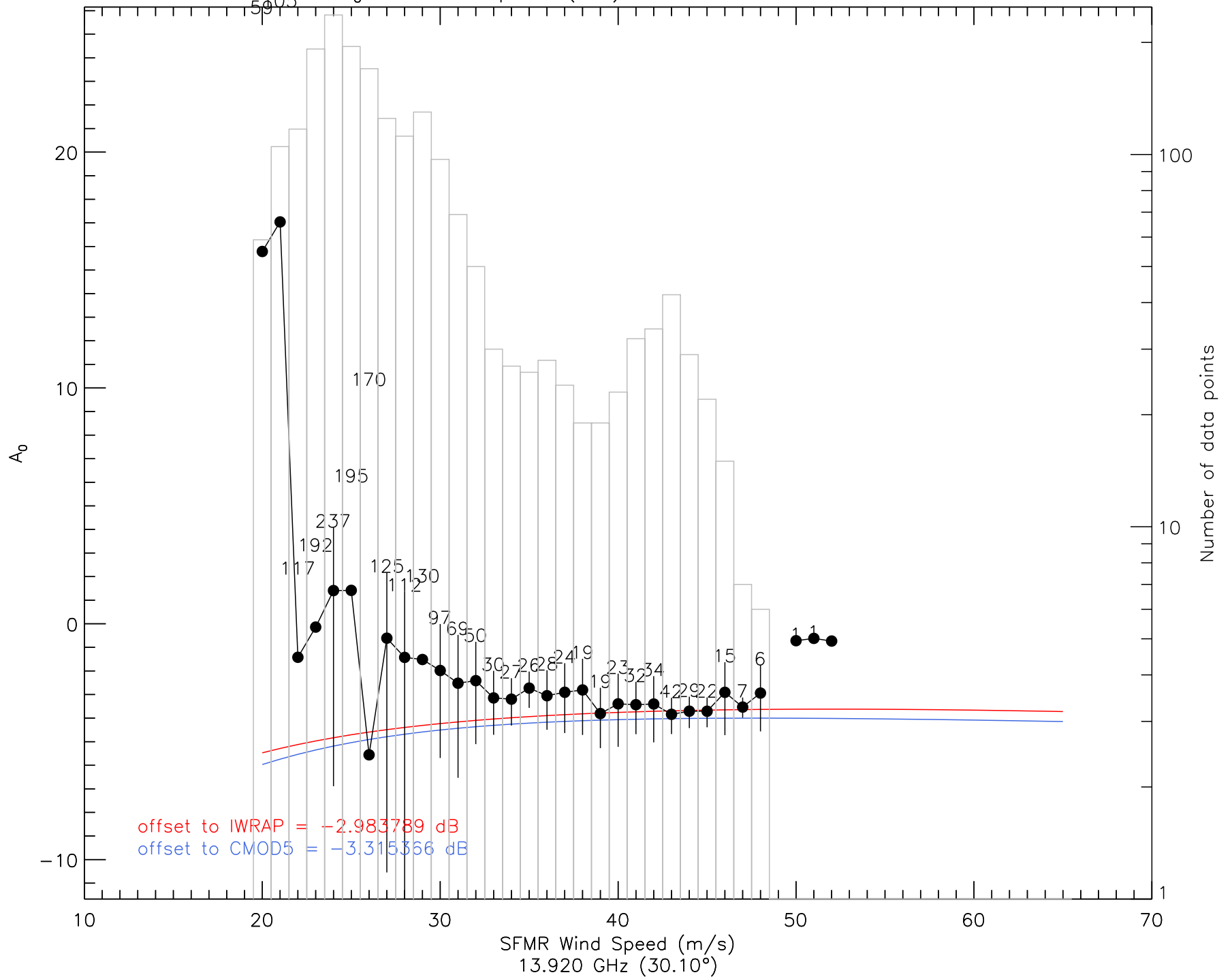
A_0 vs. Wind Speed (12a) – ku2 20080831 hws
