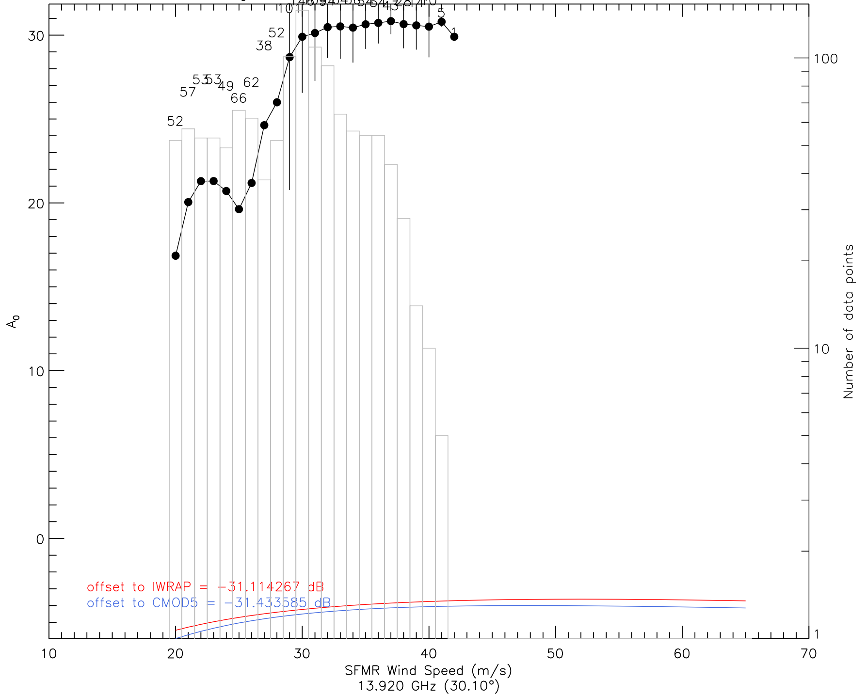
A_0 vs. Wind Speed (12a) - ku2 20080829 hws
