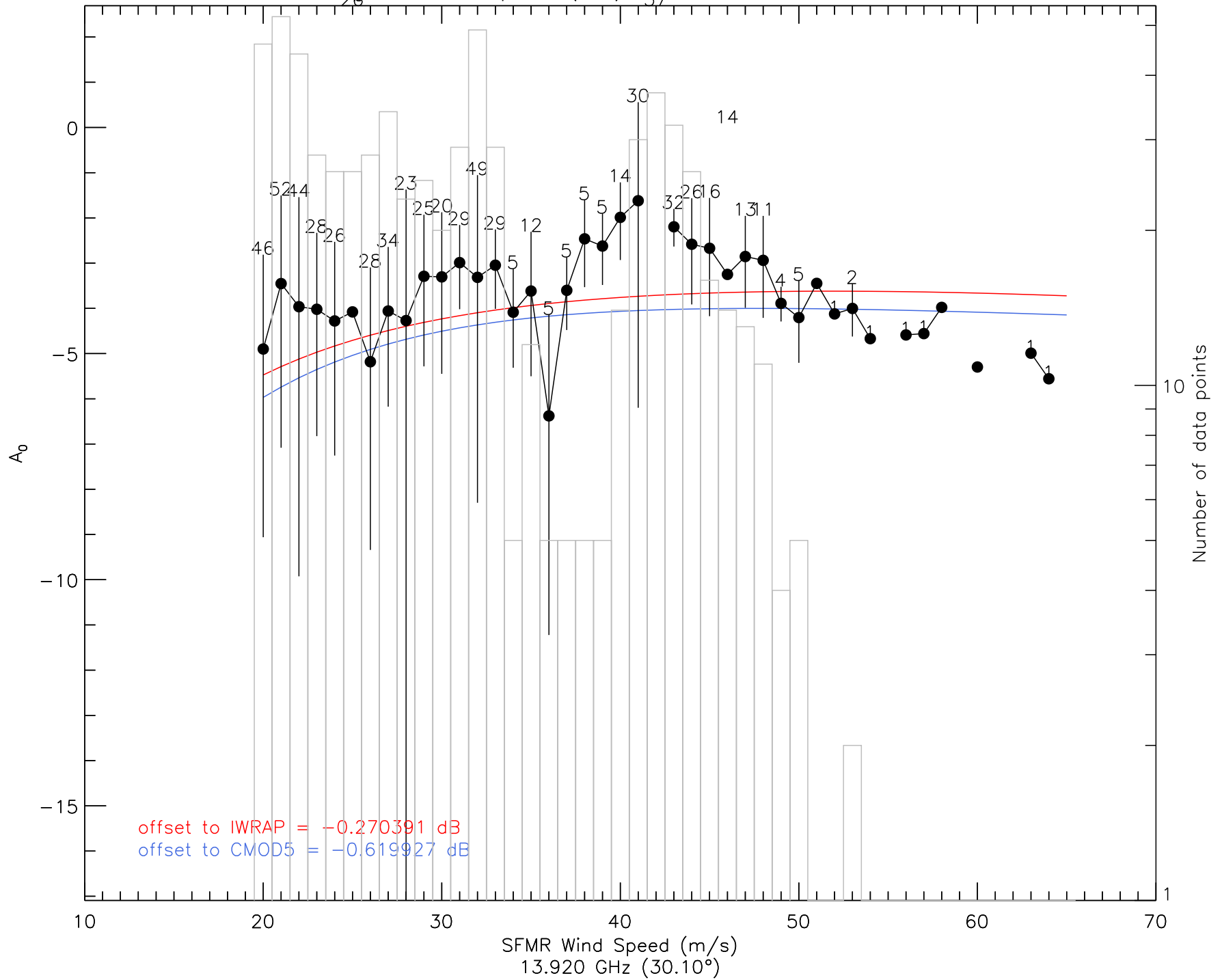
A_0 vs. Wind Speed (12a) _{37}^{58} ku2 20080907 hws
