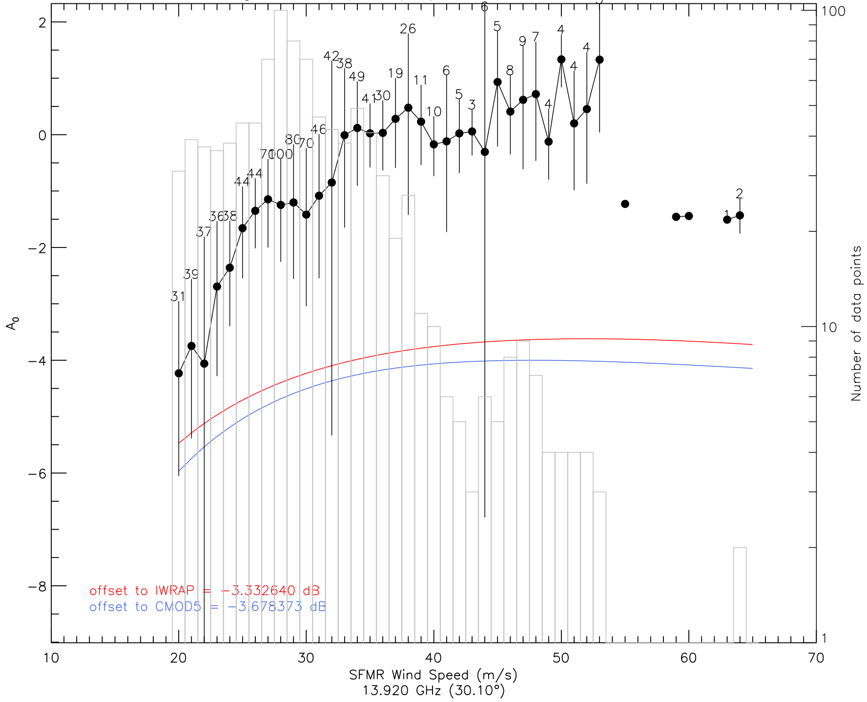
A_0 vs. Wind Speed (12a) – ku2 20080906_hws
