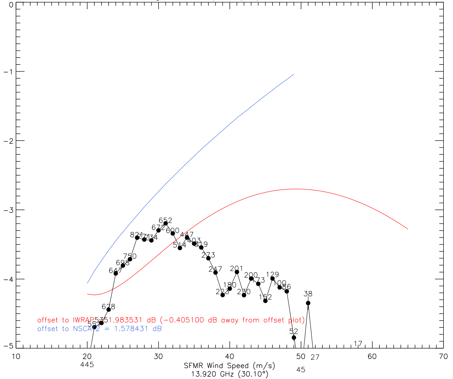
A_0 vs. Wind Speed (I2a) – All ku2
