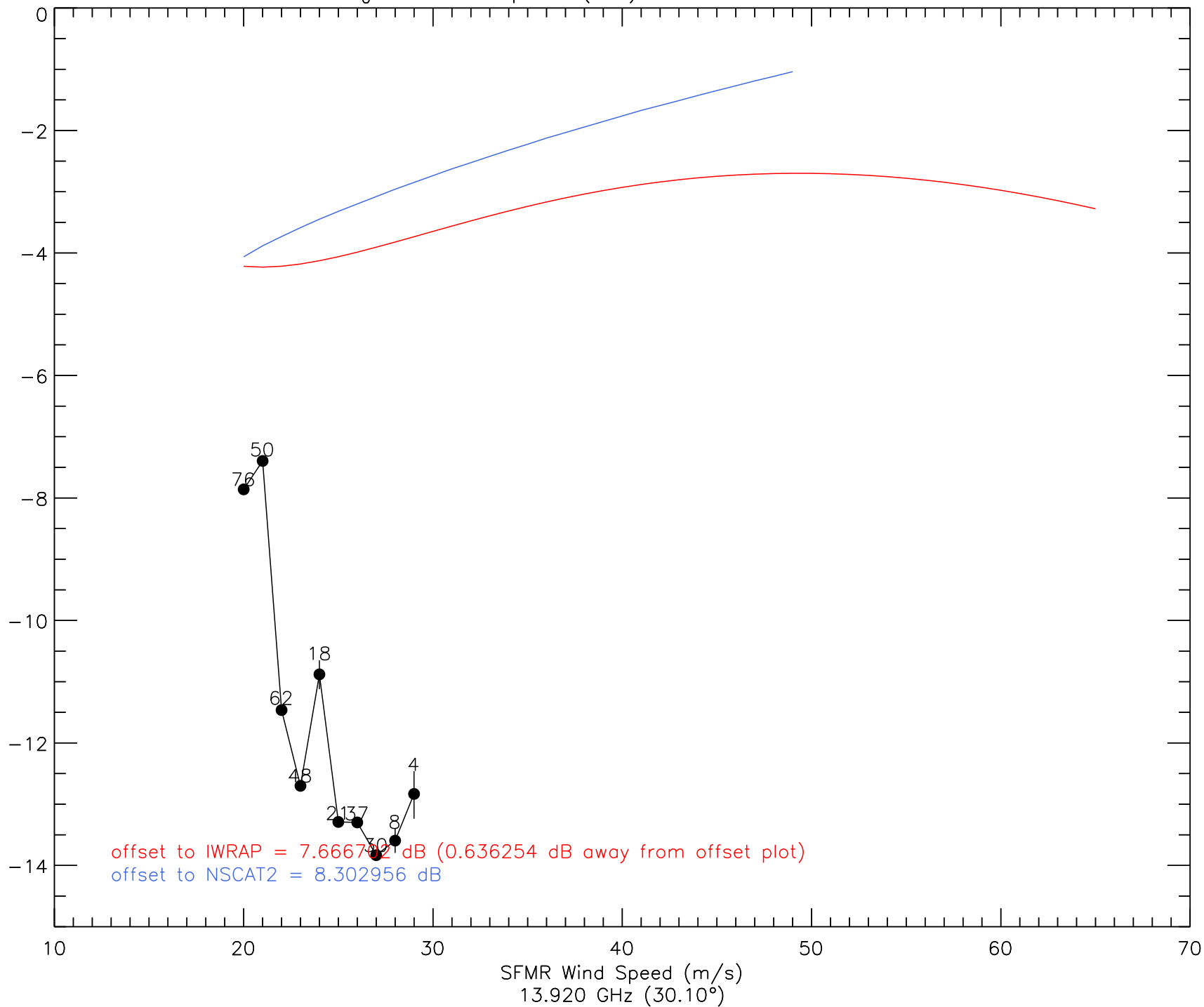
A_0 vs. Wind Speed (I2a) - 20080925 - ku2
