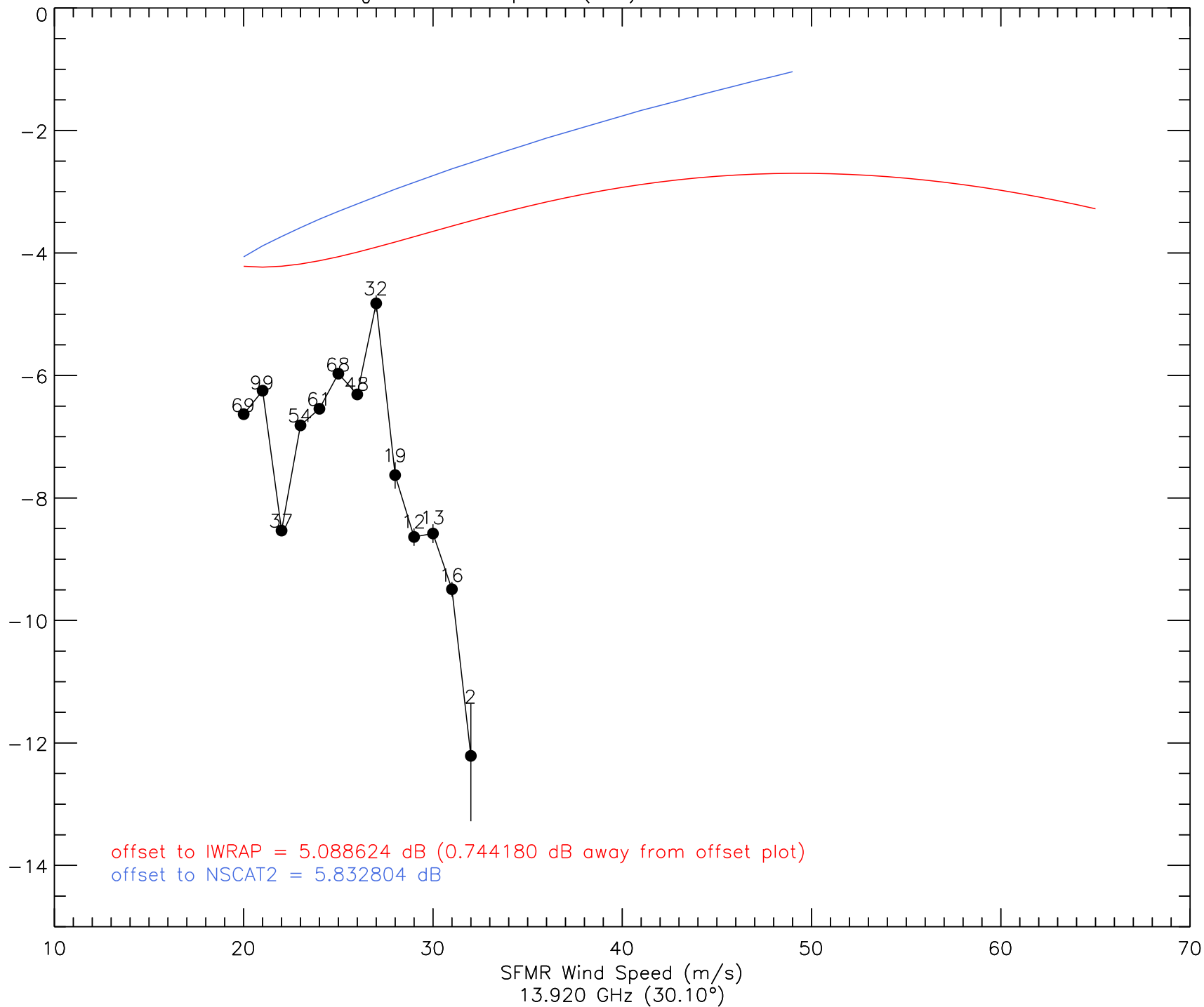
A_0 vs. Wind Speed (I2a) - 20080909 - ku2
