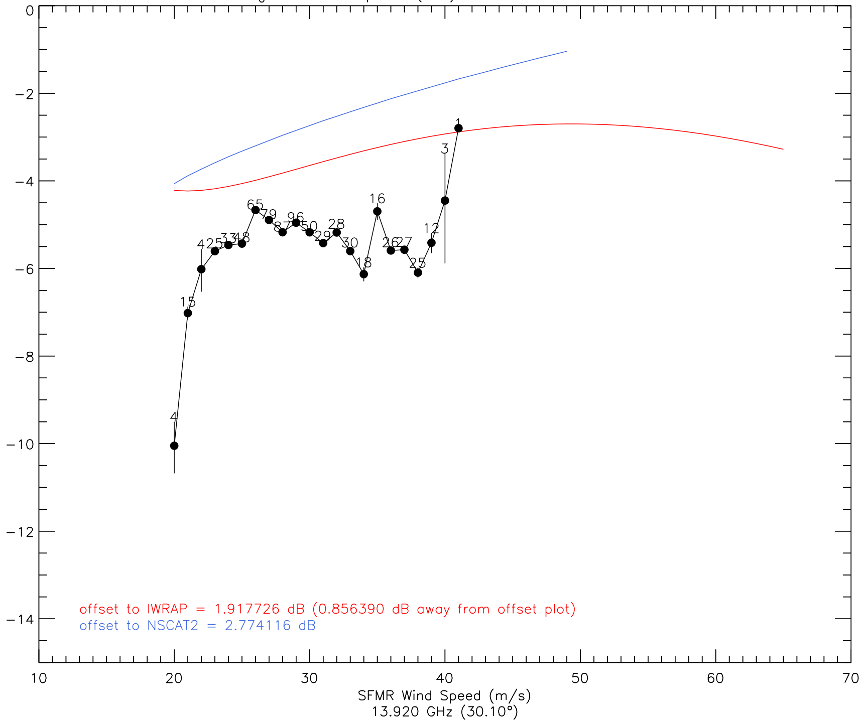
A_0 vs. Wind Speed (I2a) - 20080911 - ku2
