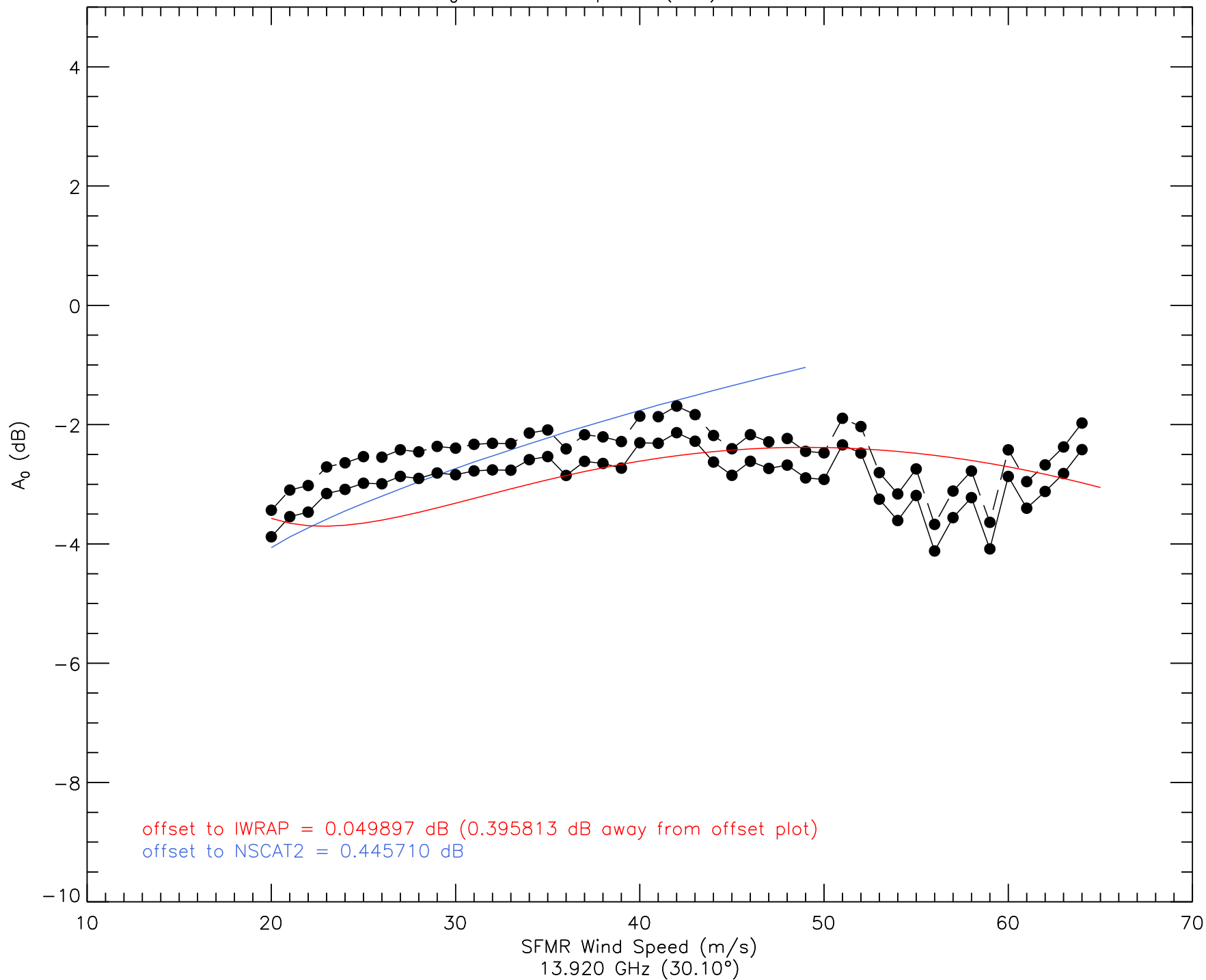
A_0 vs. Wind Speed (I1b) - All ku2
