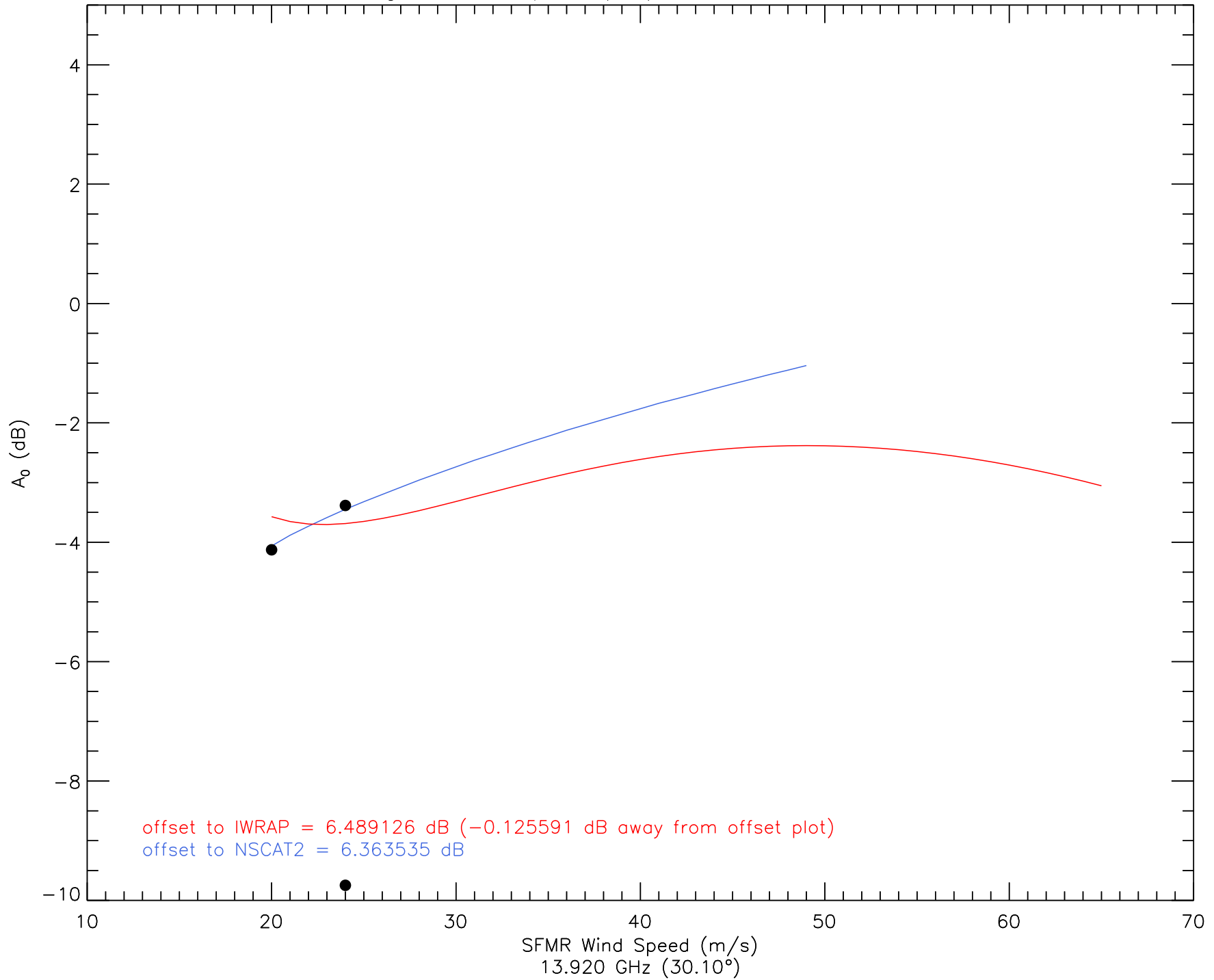
A_0 vs. Wind Speed (I1b) - 20080923 - ku2
