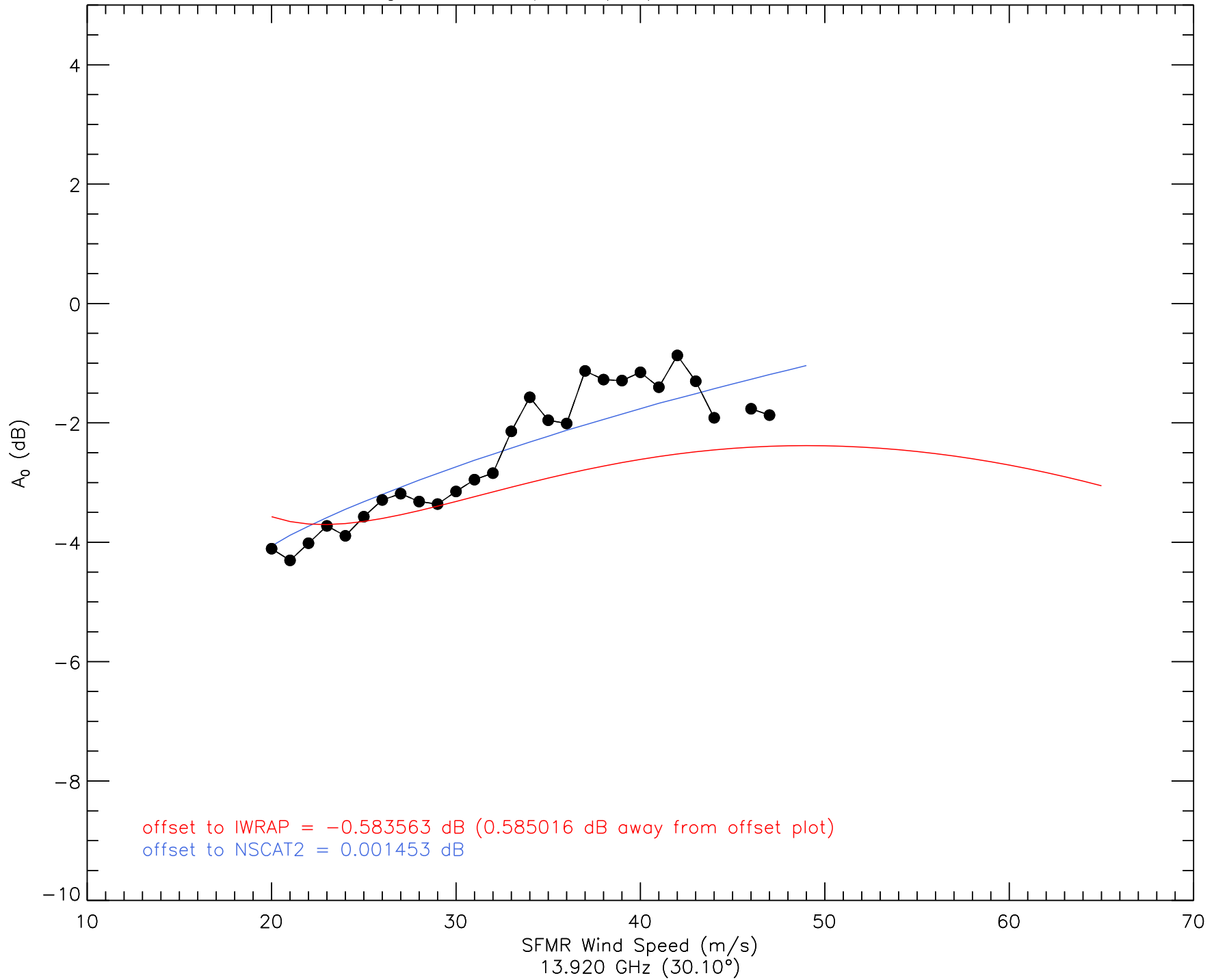
A_0 vs. Wind Speed (I1b) - 20080830 - ku2
