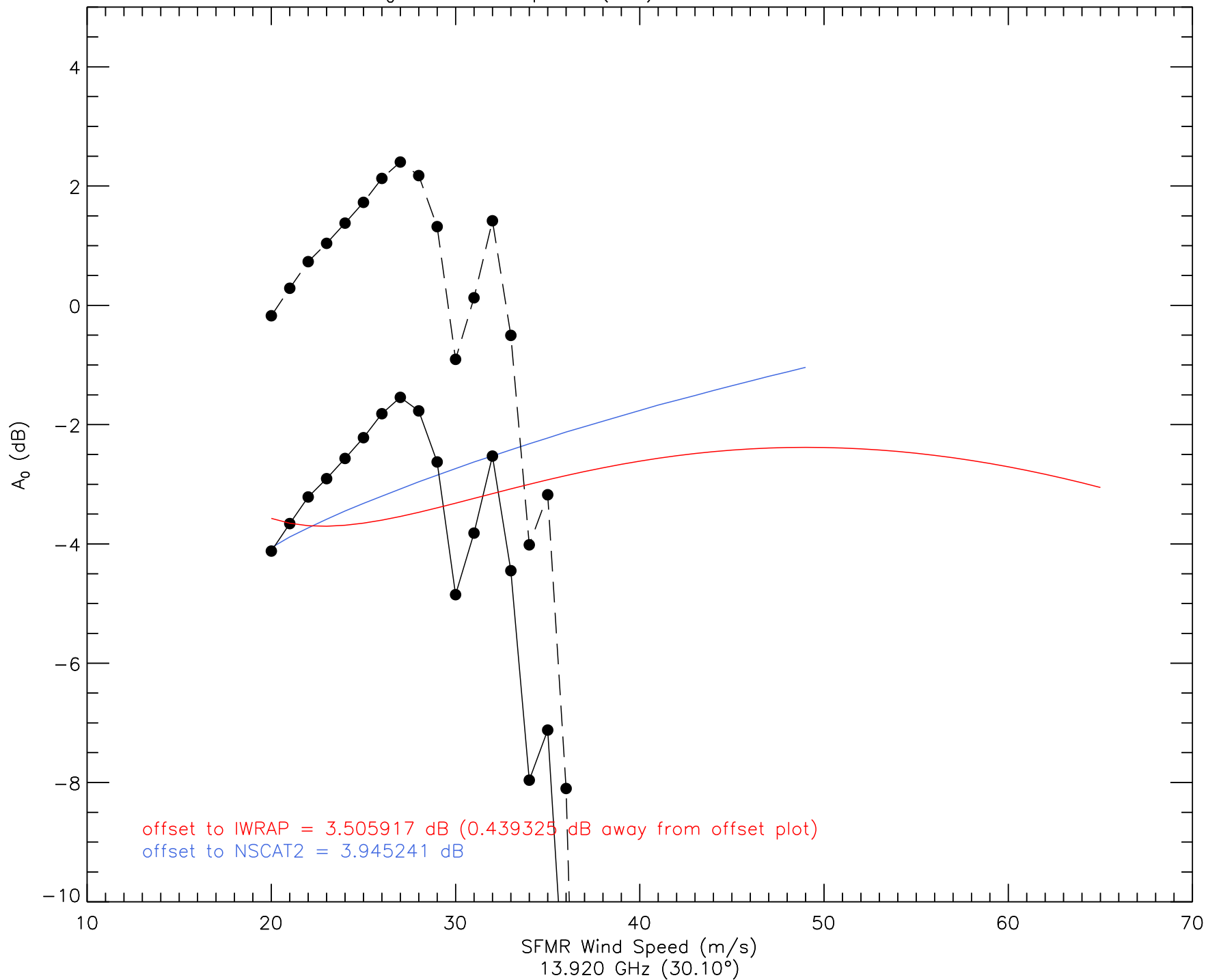
A_0 vs. Wind Speed (I1b) - 20080829 - ku2
