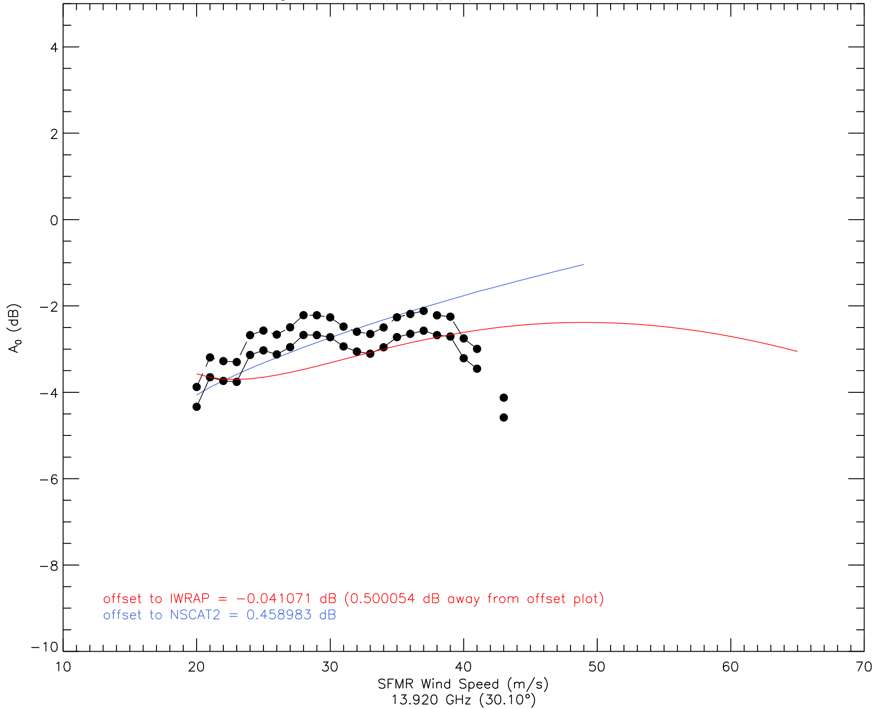
A_0 vs. Wind Speed (I1b) - 20080912 - ku2
