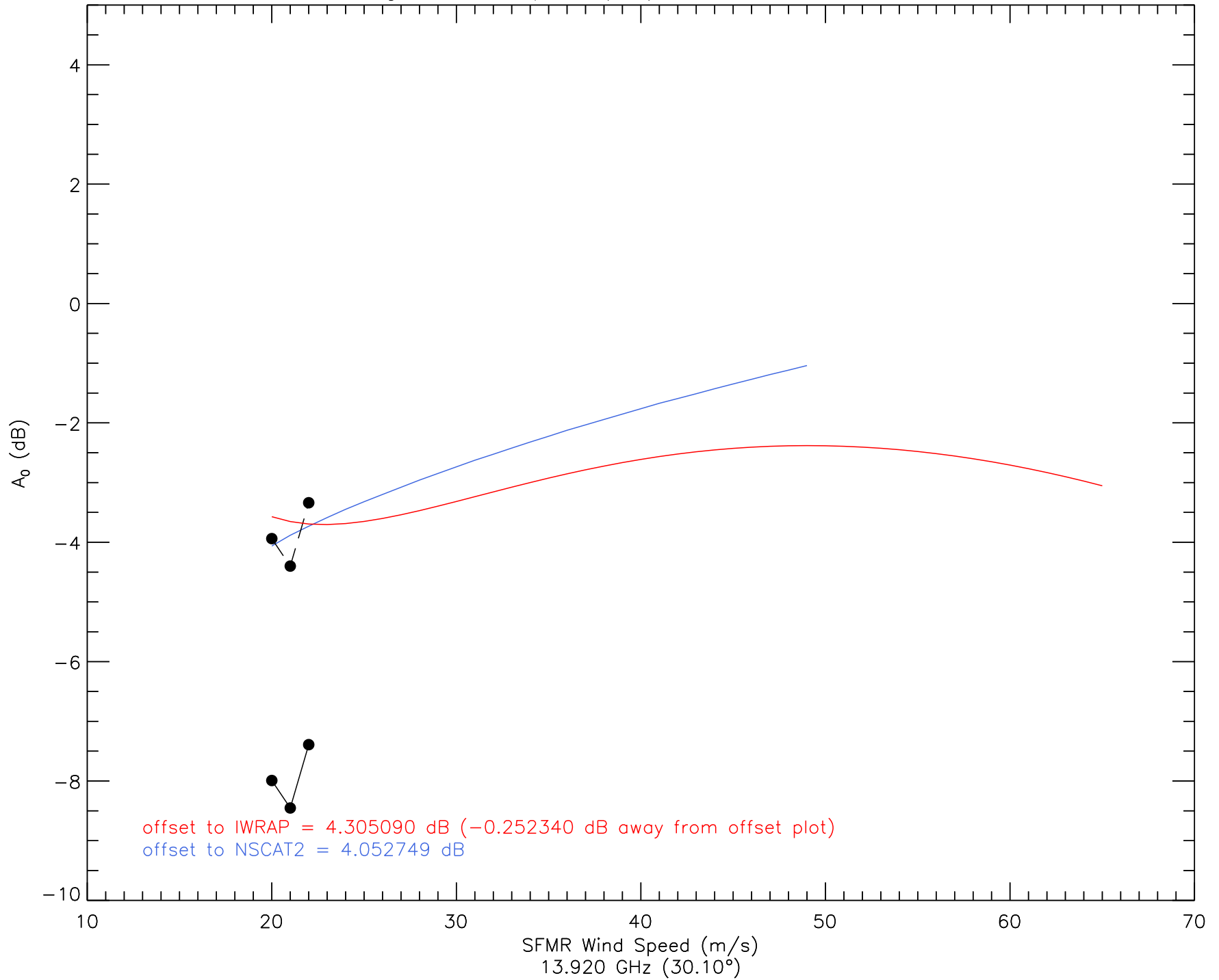
A_0 vs. Wind Speed (I1b) - 20080924 - ku2
