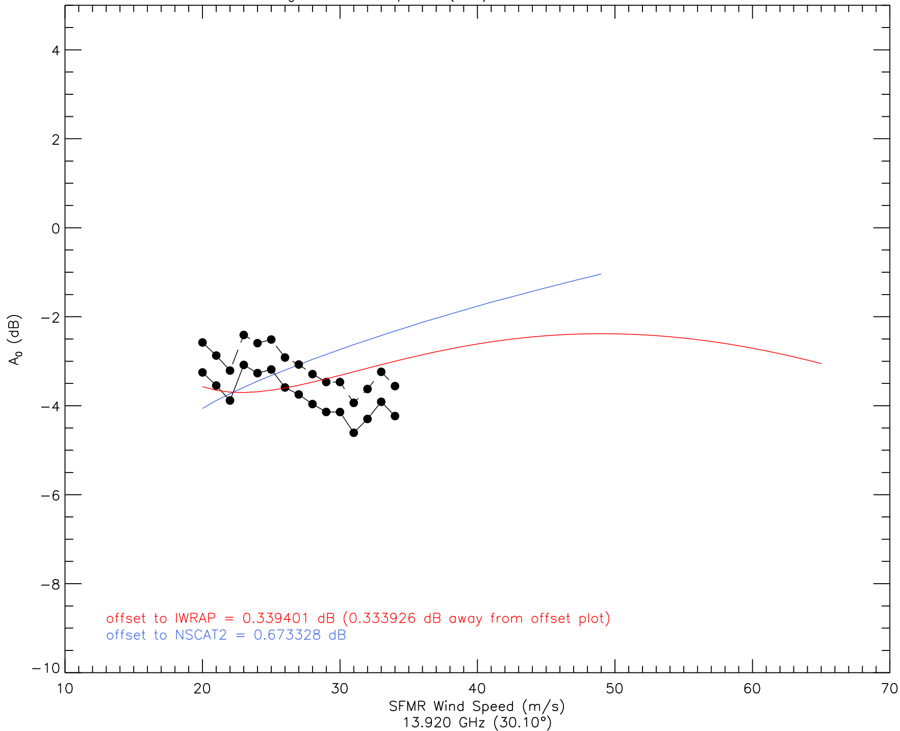
A_0 vs. Wind Speed (I1b) - 20080909 - ku2
