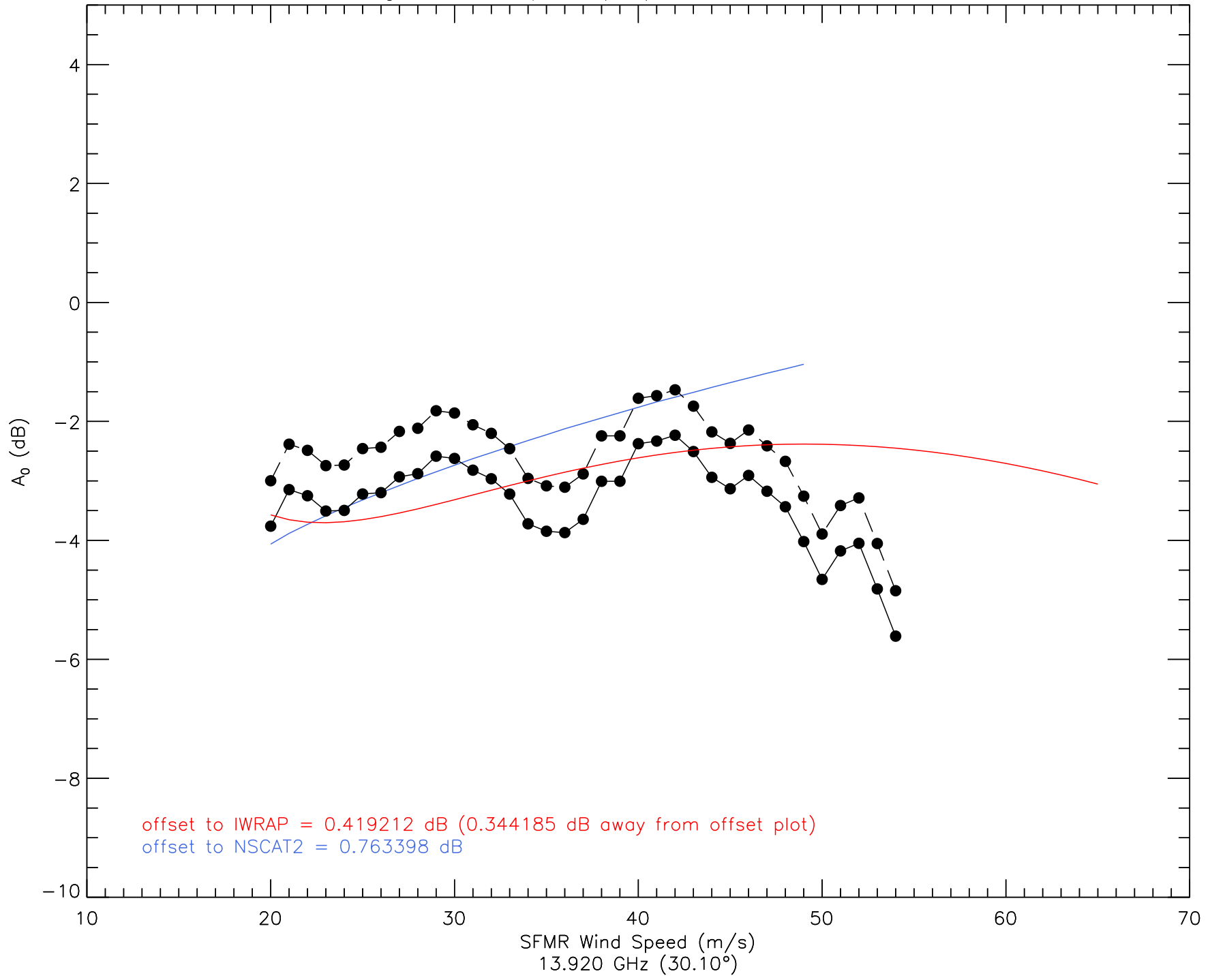
A_0 vs. Wind Speed (I1b) - 20080907 - ku2
