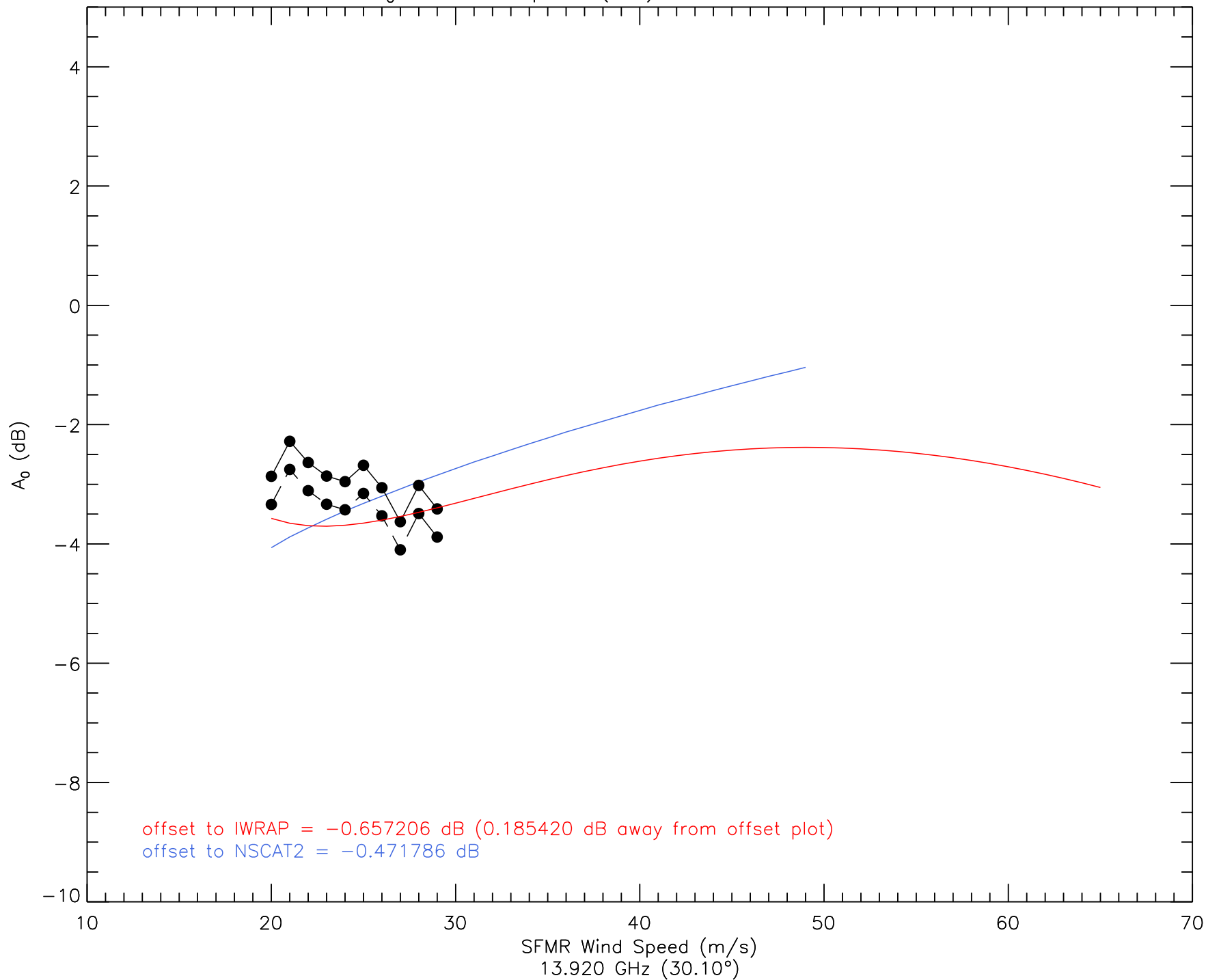
A_0 vs. Wind Speed (I1b) - 20080925 - ku2
