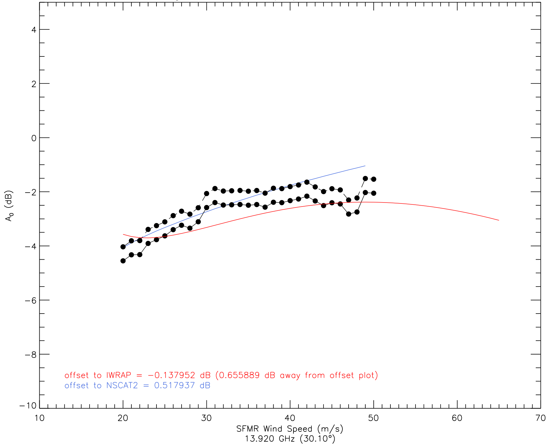
A_0 vs. Wind Speed (I1b) - 20080831 - ku2
