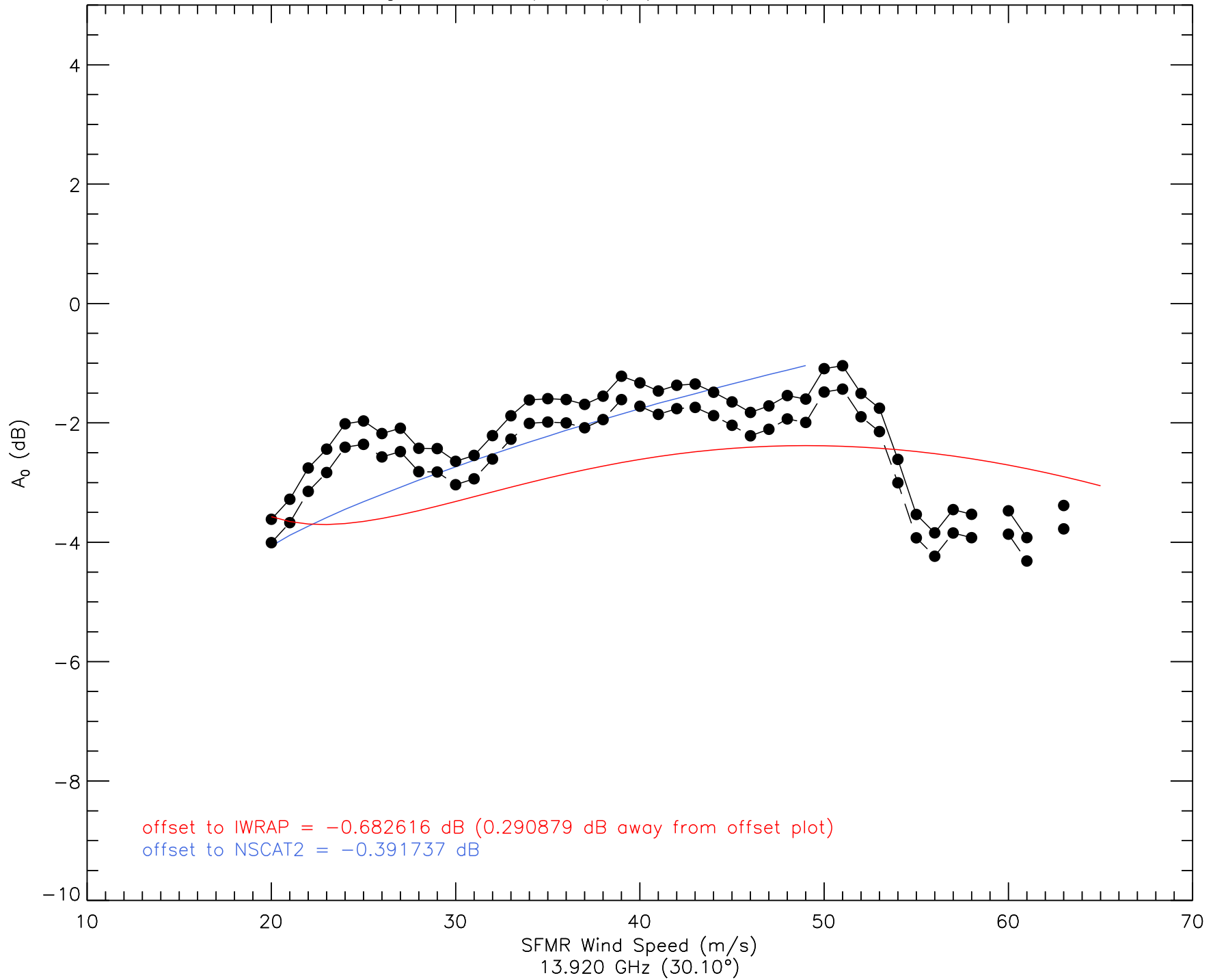
A_0 vs. Wind Speed (I1b) - 20080906 - ku2
