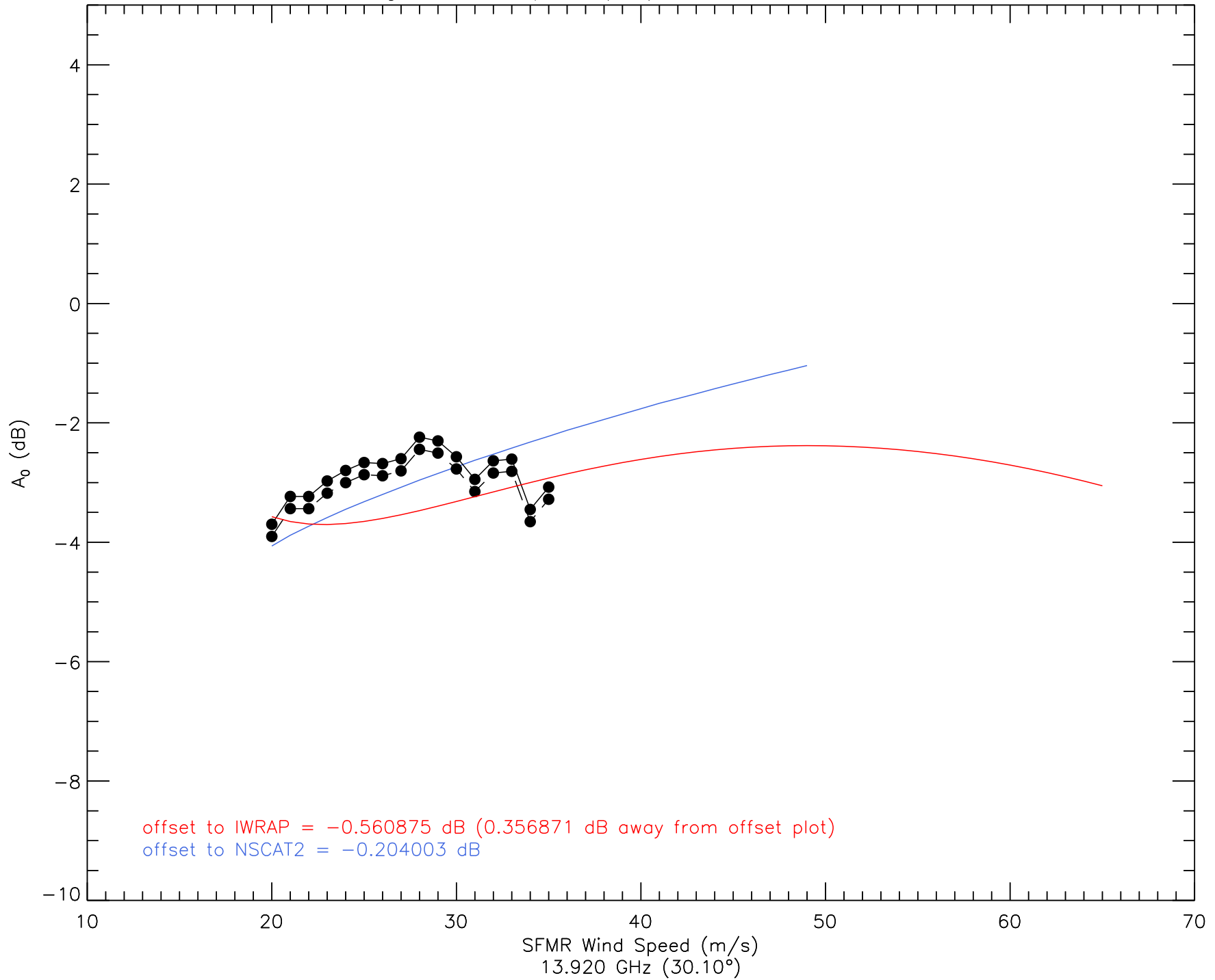
A_0 vs. Wind Speed (I1b) - 20080904 - ku2
