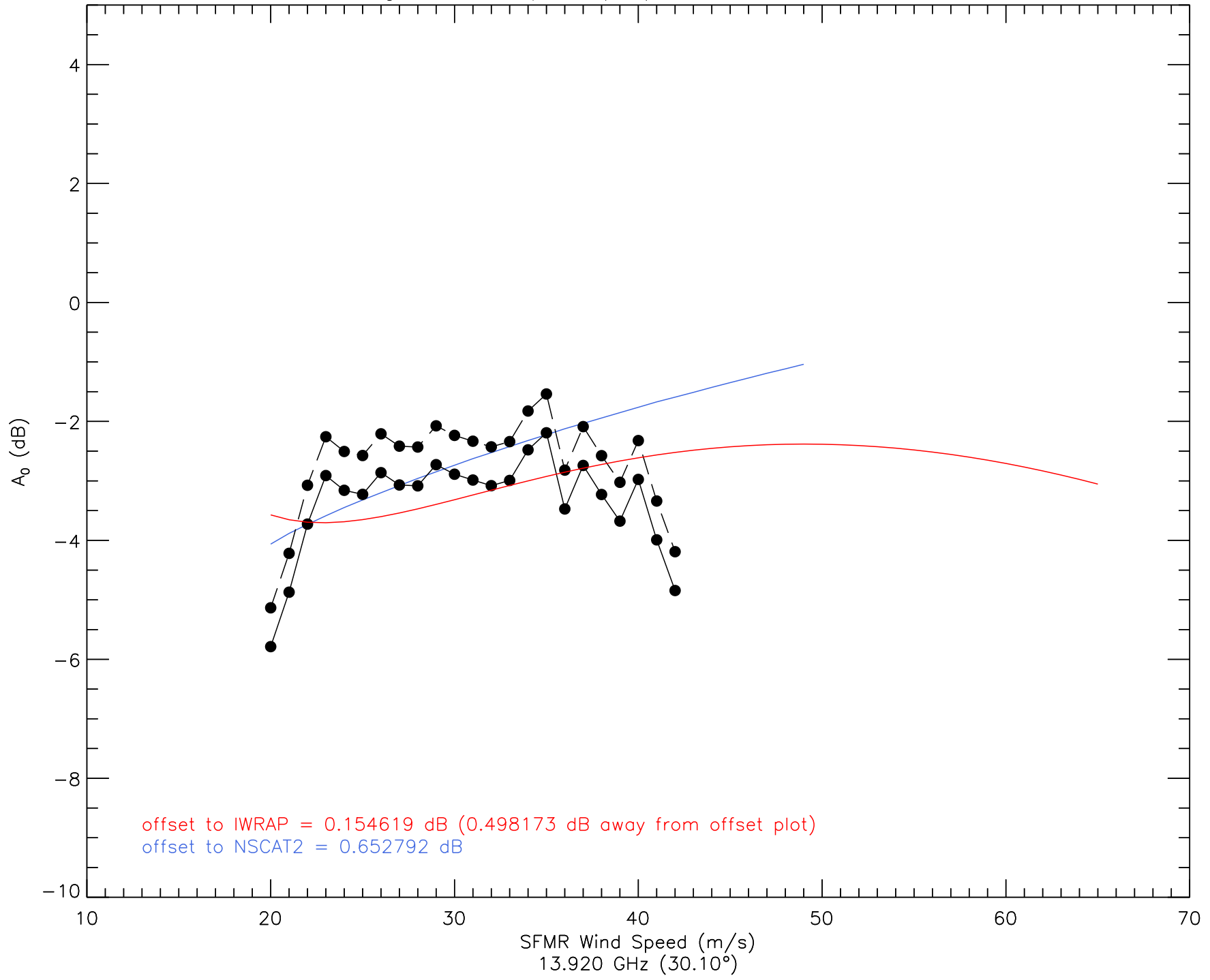
A_0 vs. Wind Speed (I1b) - 20080911 - ku2
