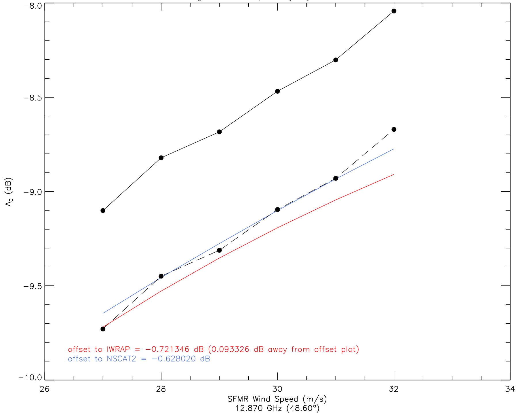
A_0 vs. Wind Speed (I1b) - All ku1
